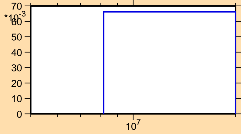
\sigma vs. E for ^{79}\text{Ga}(n,3n)
