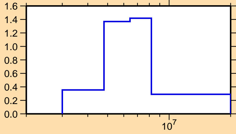
\sigma vs. E for ^{79}\text{Ga}(n,n\text{cont.})
