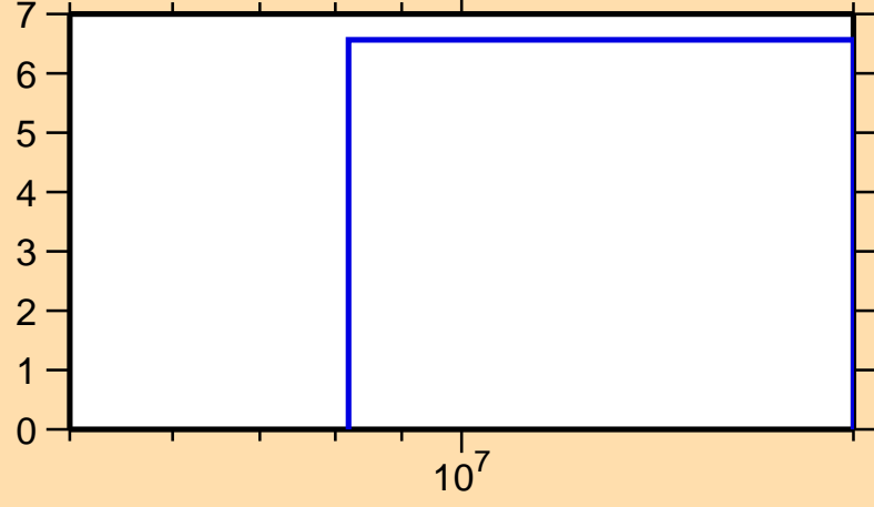
\Delta\sigma/\sigma vs. E for ^{79}\text{Ga}(n,\text{tot.})
