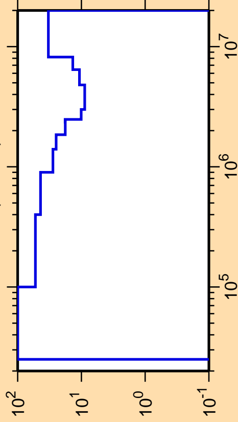
\Delta\sigma/\sigma vs. E for ^{79}\text{Ga}(n,\text{inel.})
