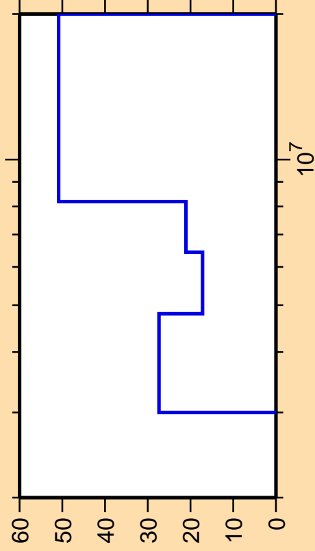
\Delta\sigma/\sigma vs. E for ^{79}\text{Ga}(n,\text{ncont.})
