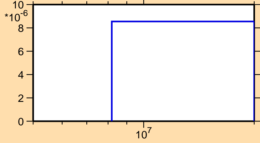
\sigma vs. E for ^{79}\text{Ga}(n,\alpha)
