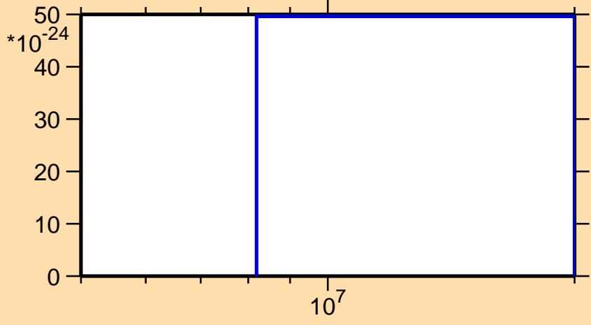
\sigma vs. E for ^{81}\text{Ga}(n,2np)
