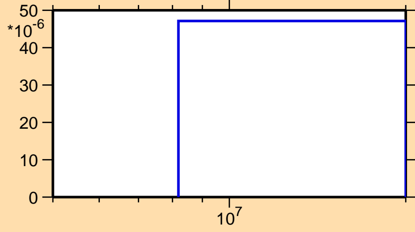
\sigma vs. E for ^{81}\text{Ga}(n,p)
