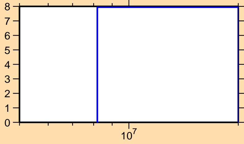
\Delta\sigma/\sigma vs. E for ^{81}\text{Ga}(n,\text{el.})
