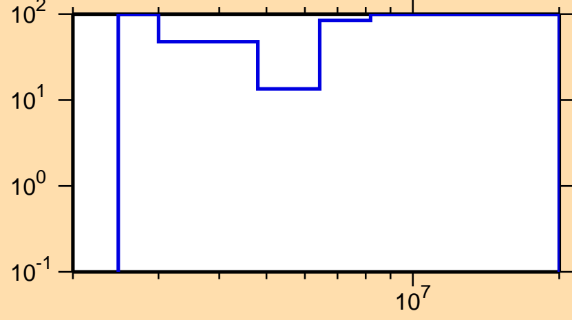
\Delta\sigma/\sigma vs. E for ^{81}\text{Ga}(n,n\text{cont.})
