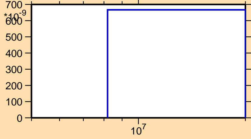
\sigma vs. E for ^{81}\text{Ga}(n,\alpha)
