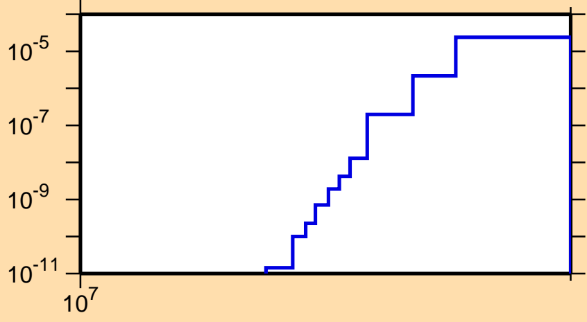
\sigma vs. E for ^{64}\text{Ge} (mt 45)
