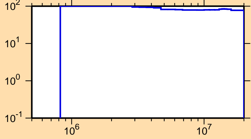
\Delta\sigma/\sigma vs. E for ^{64}\text{Ge}(n,\text{inel.})
