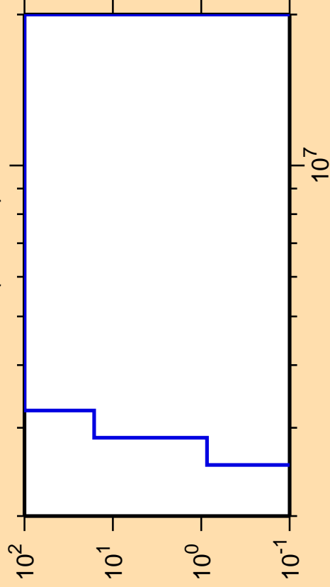
\Delta\sigma/\sigma vs. E for ^{64}\text{Ge}(n,\text{He}3)
