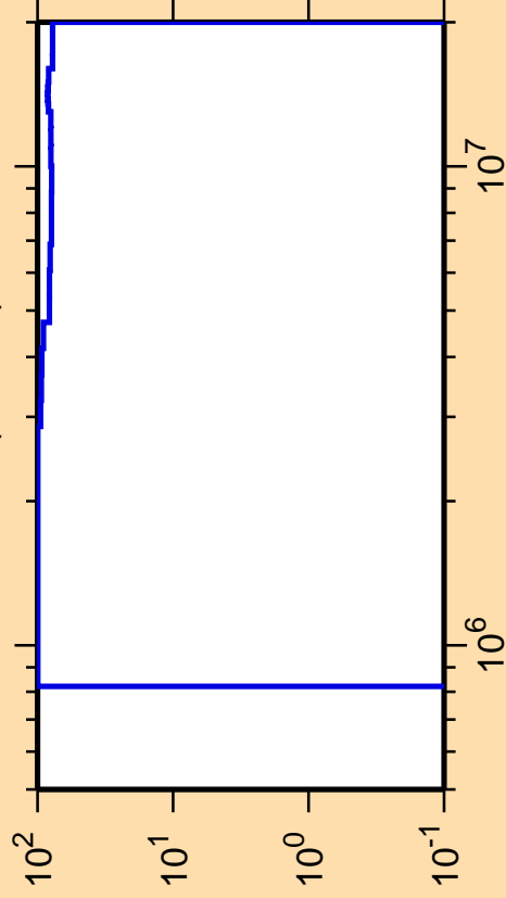
\Delta\sigma/\sigma vs. E for ^{64}\text{Ge}(n,\text{inel.})
