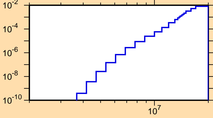
\sigma vs. E for ^{64}\text{Ge}(n,\text{He}3)
