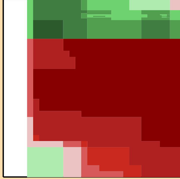
\Delta\sigma/\sigma vs. E for ^{64}\text{Ge}(n,n_1)
