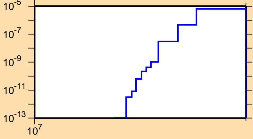
\sigma vs. E for ^{65}\text{Ge} (mt 34)
