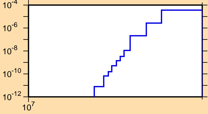
\sigma vs. E for ^{65}\text{Ge} (mt 45)
