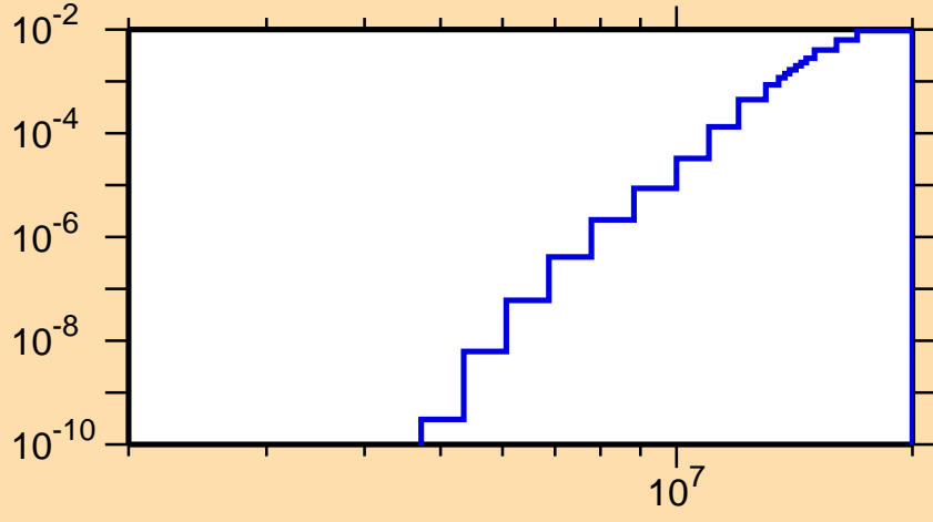
\sigma vs. E for ^{65}\text{Ge}(n,\text{He}3)
