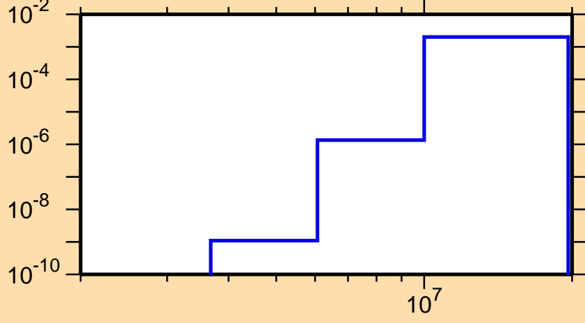
\sigma vs. E for ^{65}\text{Ge}(n,\text{He}3)
