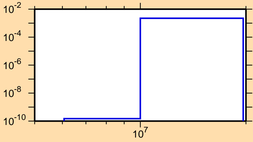
\sigma vs. E for ^{65}\text{Ge}(n,pd)
