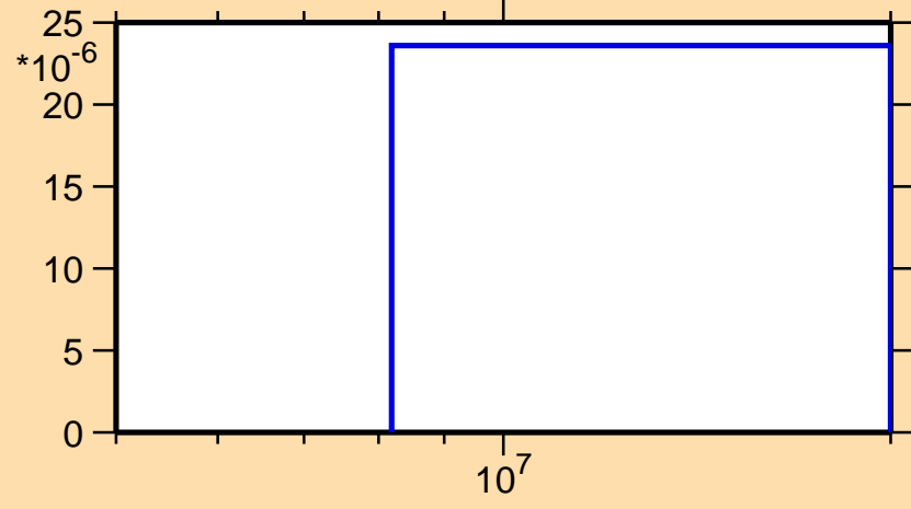
\sigma vs. E for ^{65}\text{Ge}(n,\text{pt})
