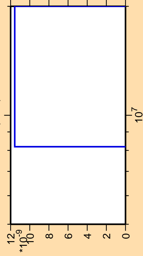
\Delta\sigma/\sigma vs. E for ^{65}\text{Ge}(n,nt)
