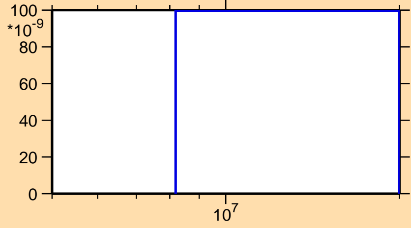
\sigma vs. E for ^{65}\text{Ge}(n,\text{nd})
