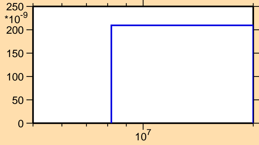
\sigma vs. E for ^{65}\text{Ge}(\text{mt117})
