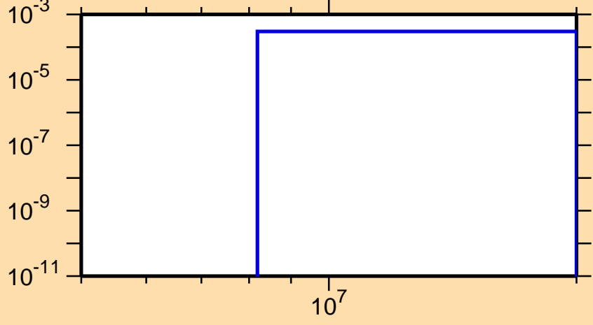
\sigma vs. E for ^{65}\text{Ge}(n,t)
