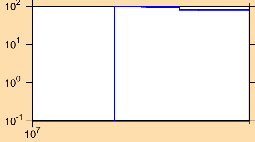
\Delta\sigma/\sigma vs. E for ^{66}\text{Ge}(n,2n)
