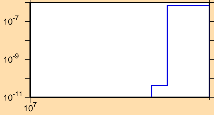
\sigma vs. E for ^{66}\text{Ge}(n,\text{pt})
