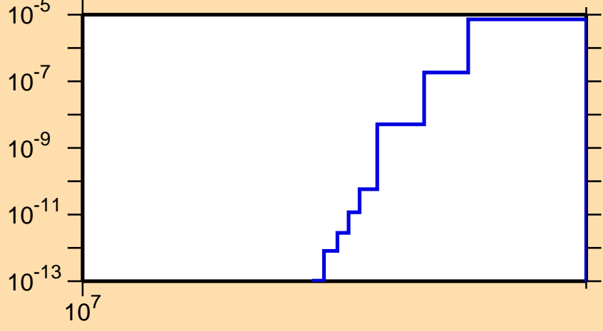
\sigma vs. E for ^{66}\text{Ge} (mt 45)
