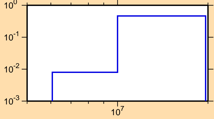
\sigma vs. E for ^{66}\text{Ge}(n,np)
