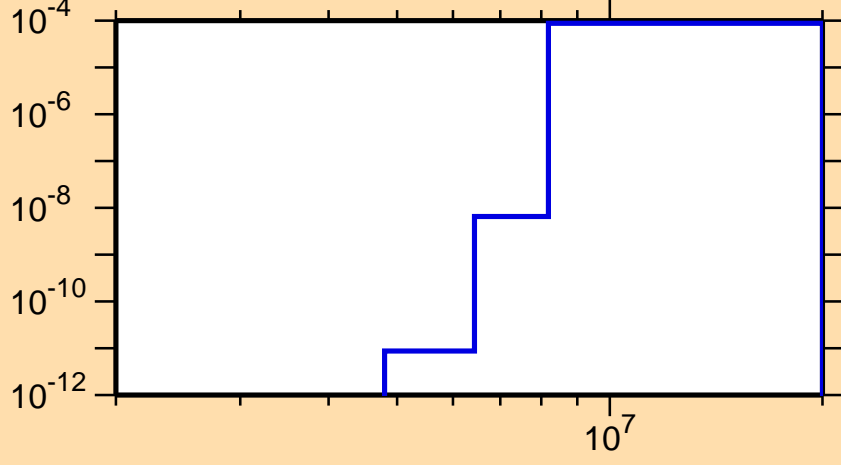
\sigma vs. E for ^{66}\text{Ge}(n,\text{He}3)
