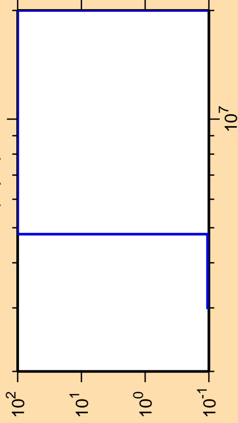
\Delta\sigma/\sigma vs. E for ^{66}\text{Ge}(n,p\alpha)
