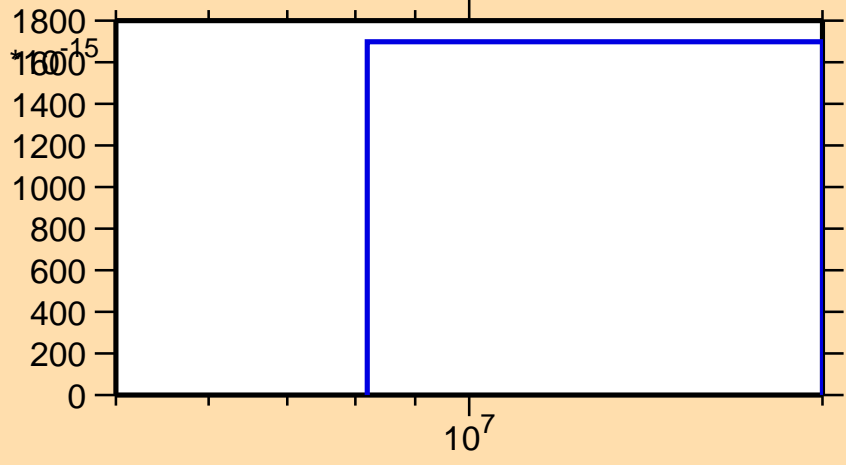
\sigma vs. E for ^{66}\text{Ge} (mt 34)
