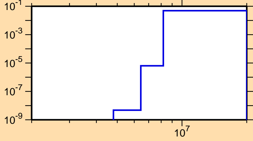
\sigma vs. E for ^{66}\text{Ge}(n,p\alpha)
