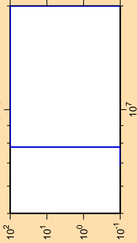
\Delta\sigma/\sigma vs. E for ^{67}\text{Ge}(n,t)
