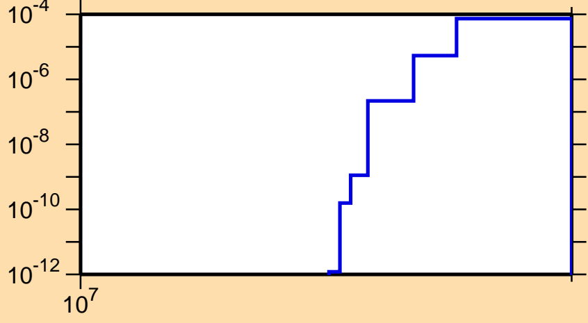
\sigma vs. E for ^{67}\text{Ge}(n,nd)
