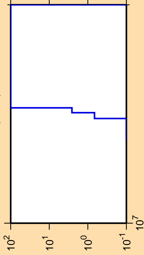
\Delta\sigma/\sigma vs. E for ^{67}\text{Ge}(n,nd)
