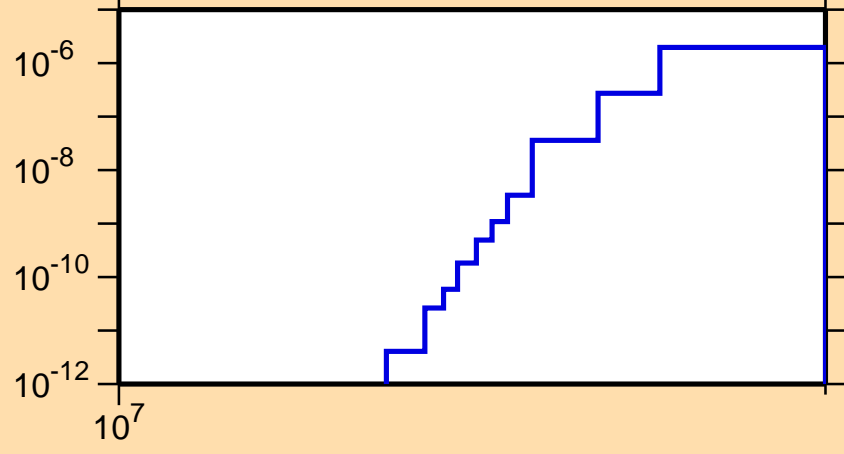
\sigma vs. E for ^{67}\text{Ge}(\text{mt117})
