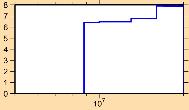
\Delta\sigma/\sigma vs. E for ^{67}\text{Ge}(n,\text{nonel.})
