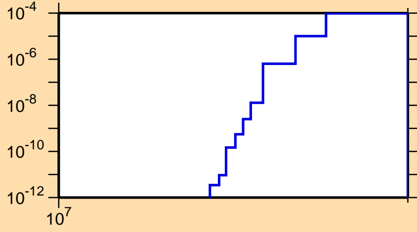
\sigma vs. E for ^{67}\text{Ge}(n,\text{pt})
