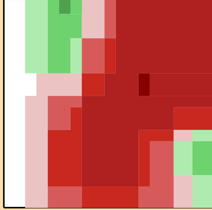
\Delta\sigma/\sigma vs. E for ^{67}\text{Ge}(n,n\text{cont.})
