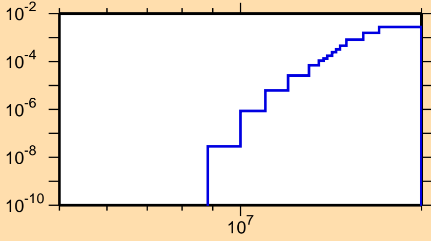
\sigma vs. E for ^{67}\text{Ge}(n,t)
