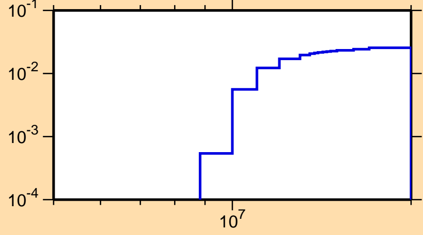
\sigma vs. E for ^{67}\text{Ge}(n,2n)
