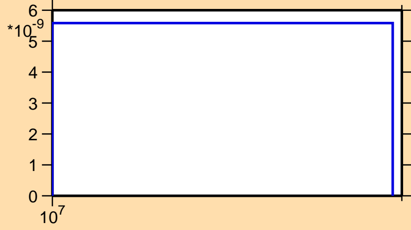
\sigma vs. E for ^{67}\text{Ge} (mt 34)
