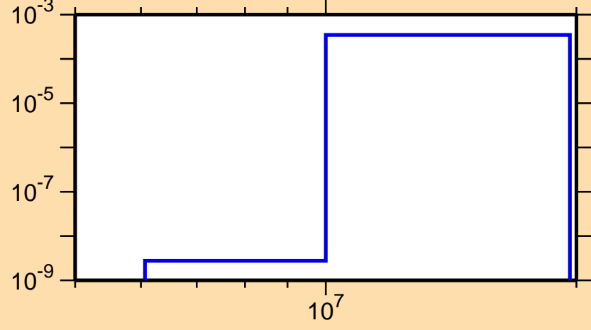
\sigma vs. E for ^{67}\text{Ge}(n,t)
