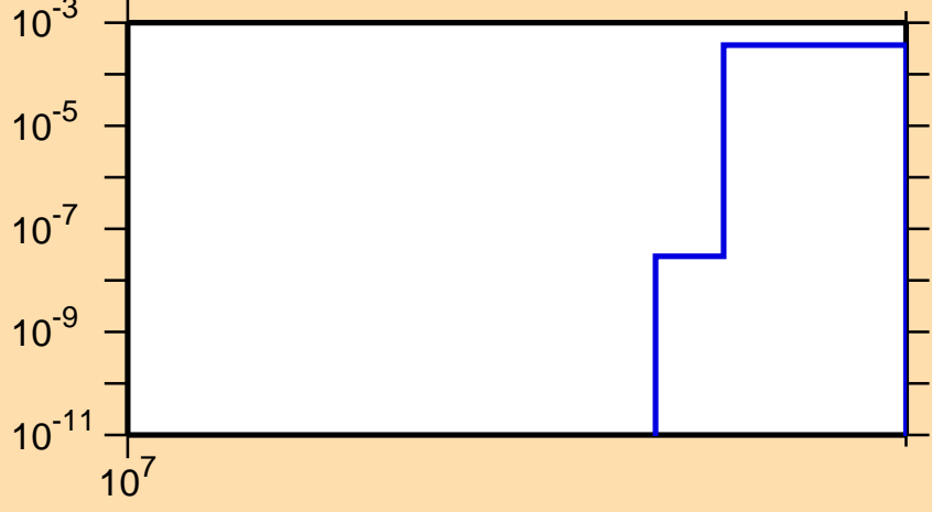
\sigma vs. E for ^{69}\text{Ge}(n,2np)
