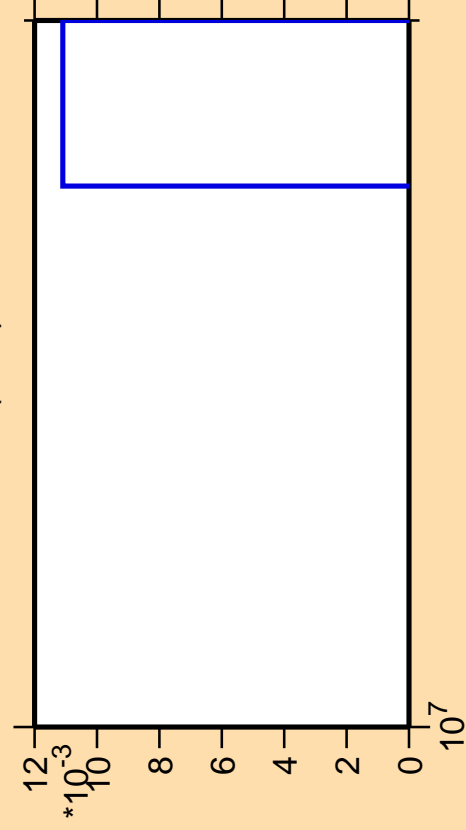
\Delta\sigma/\sigma vs. E for ^{69}\text{Ge}(n,nt)
