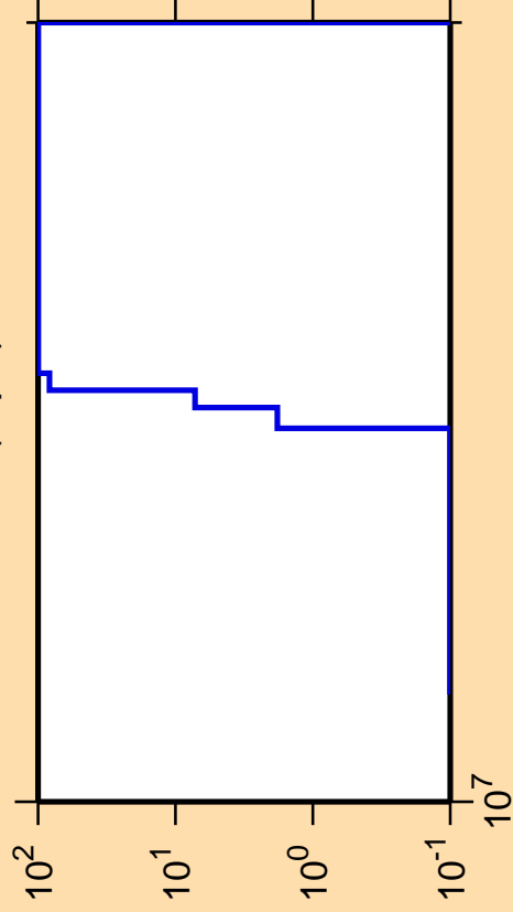
\Delta\sigma/\sigma vs. E for ^{69}\text{Ge}(n,pd)
