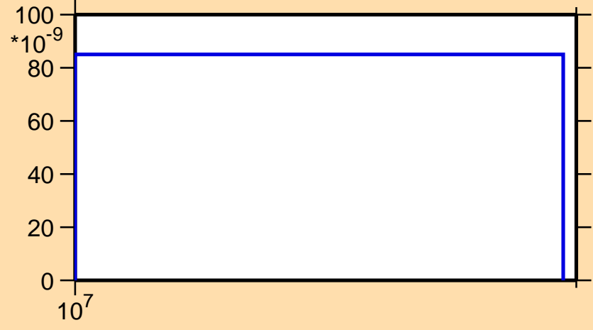
\sigma vs. E for ^{69}\text{Ge}(n,\text{pd})
