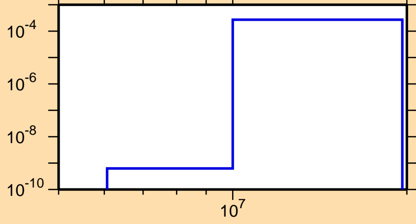
\sigma vs. E for ^{69}\text{Ge}(n,t)
