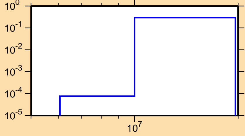
\sigma vs. E for ^{69}\text{Ge}(n,np)
