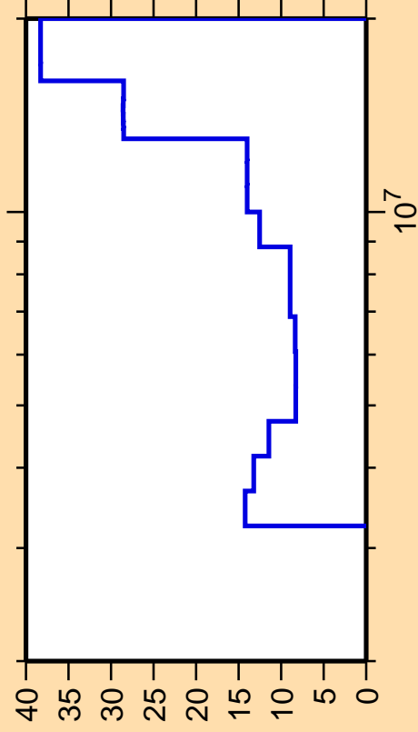
\Delta\sigma/\sigma vs. E for ^{70}\text{Ge}(n,\text{ncont.})
