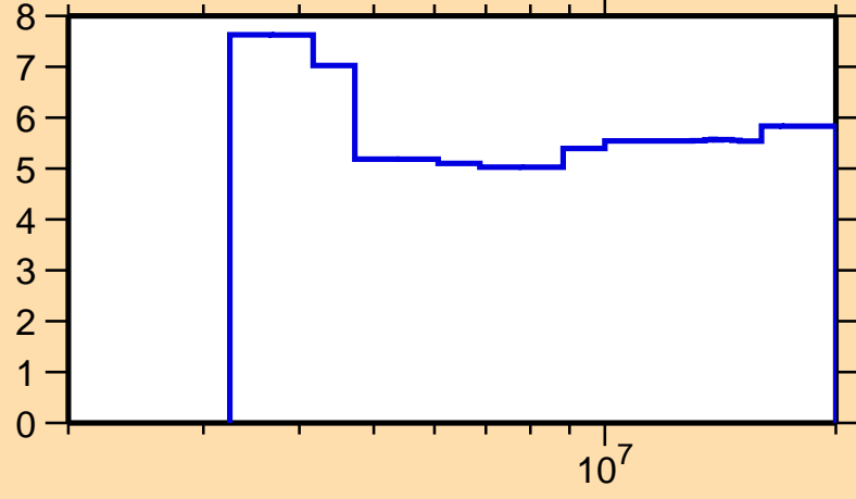
\Delta\sigma/\sigma vs. E for ^{70}\text{Ge}(n,\text{nonel.})
