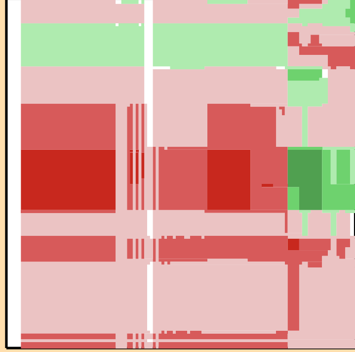
\Delta\sigma/\sigma vs. E for ^{70}\text{Ge}(n,\text{nonel.})
