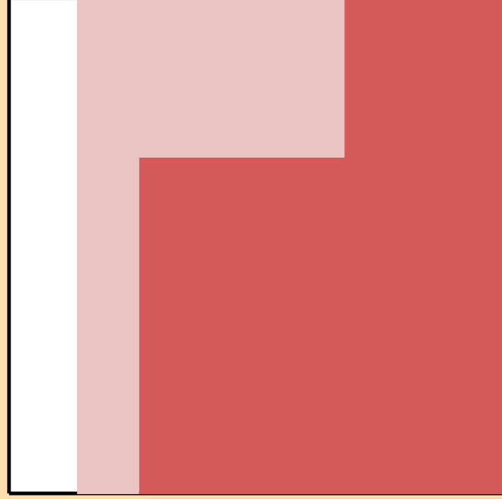
\Delta\sigma/\sigma vs. E for ^{70}\text{Ge}(n,2n)
