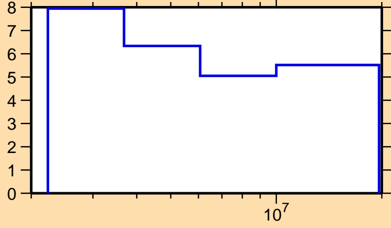
\Delta\sigma/\sigma vs. E for ^{70}\text{Ge}(n,n\text{onel.})
