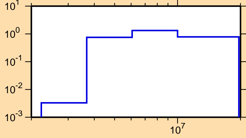
\sigma vs. E for ^{70}\text{Ge}(n,n\text{cont.})
