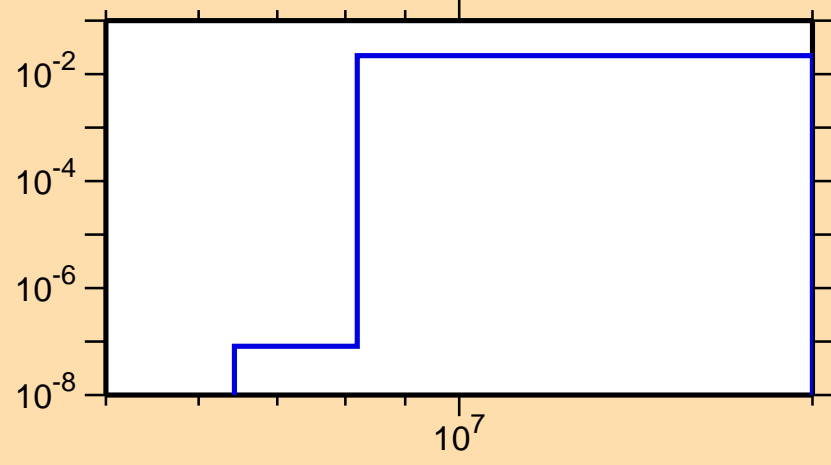
\sigma vs. E for ^{70}\text{Ge}(n,n\alpha)
