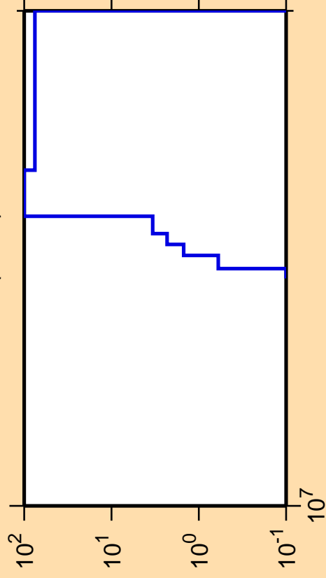
\Delta\sigma/\sigma vs. E for ^{71}\text{Ge}(n,nd)
