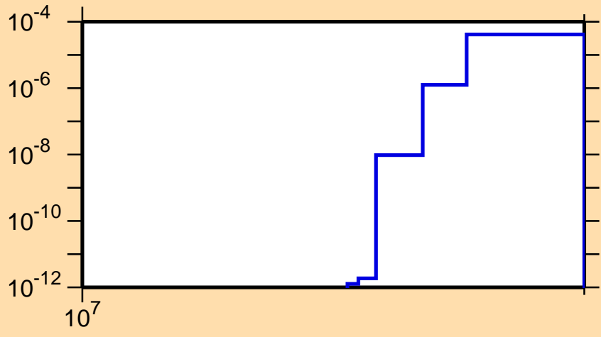
\sigma vs. E for ^{71}\text{Ge}(n,nd)
