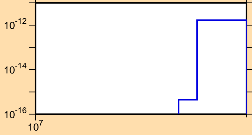
\sigma vs. E for ^{71}\text{Ge}(\text{mt117})
