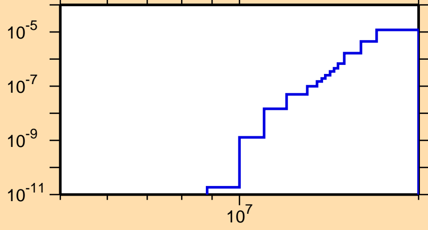
\sigma vs. E for ^{71}\text{Ge}(n,p\alpha)
