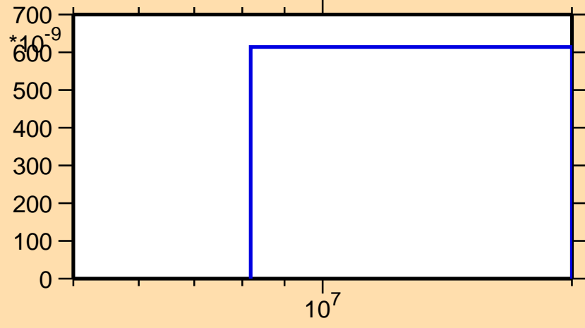
\sigma vs. E for ^{71}\text{Ge}(n,p\alpha)
