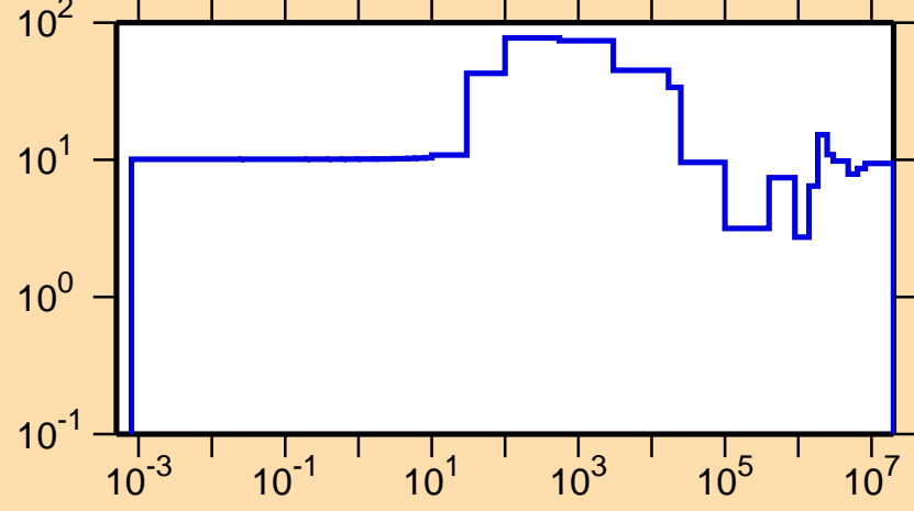
\Delta\sigma/\sigma vs. E for ^{71}\text{Ge}(n,\text{el.})
