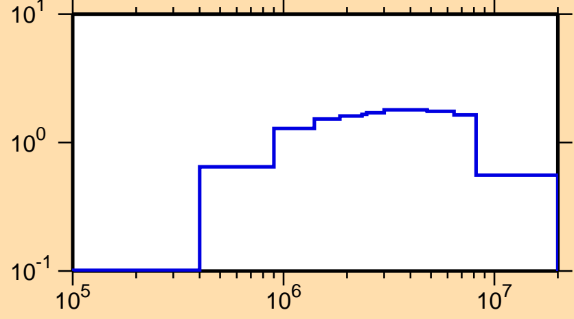
\sigma vs. E for ^{71}\text{Ge}(n,\text{inel.})
