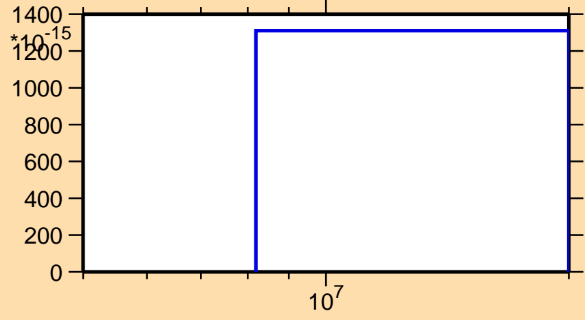
\sigma vs. E for ^{71}\text{Ge}(n,pd)
