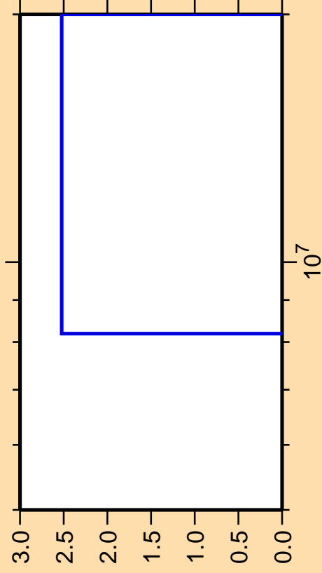
\Delta\sigma/\sigma vs. E for ^{71}\text{Ge}(n,pd)
