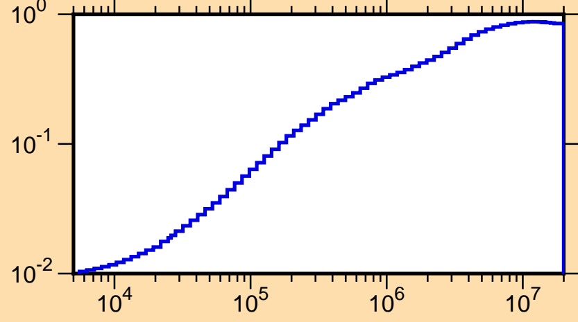
\mu vs. E for ^{74}\text{Ge}(\text{mt251})
