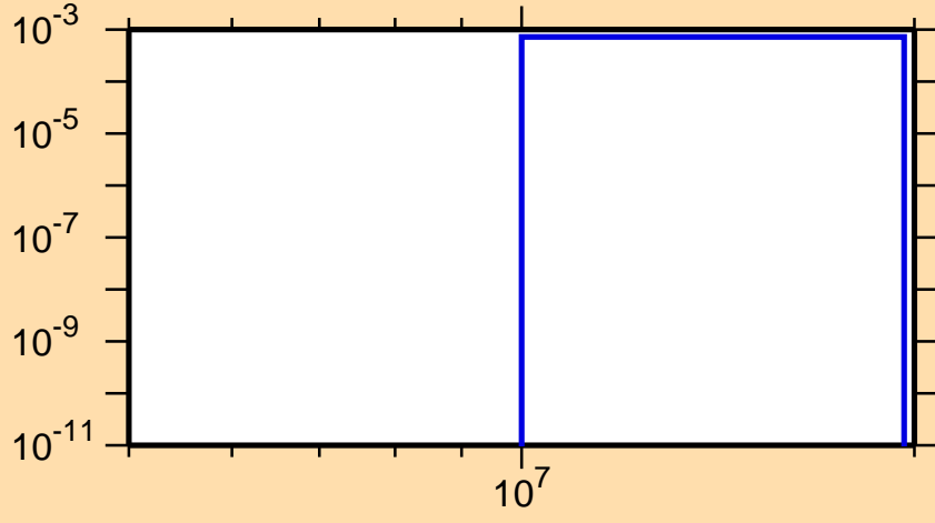
\sigma vs. E for ^{75}\text{Ge}(n,d)
