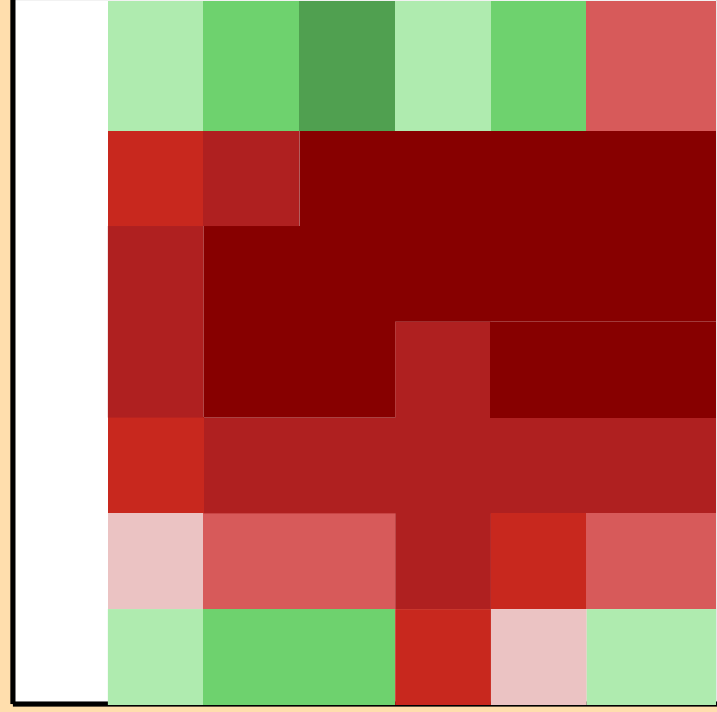
\Delta\sigma/\sigma vs. E for ^{75}\text{Ge}(n,n\text{cont.})
