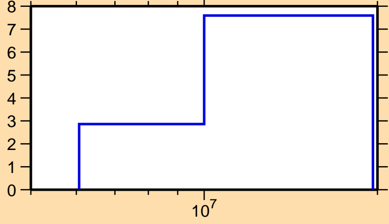
\Delta\sigma/\sigma vs. E for ^{75}\text{Ge}(n,\text{tot.})
