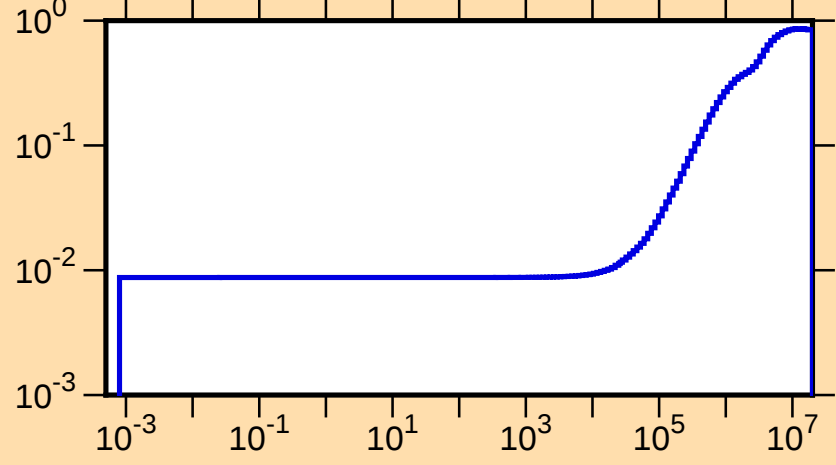
\mu vs. E for ^{77}\text{Ge}(\text{mt251})
