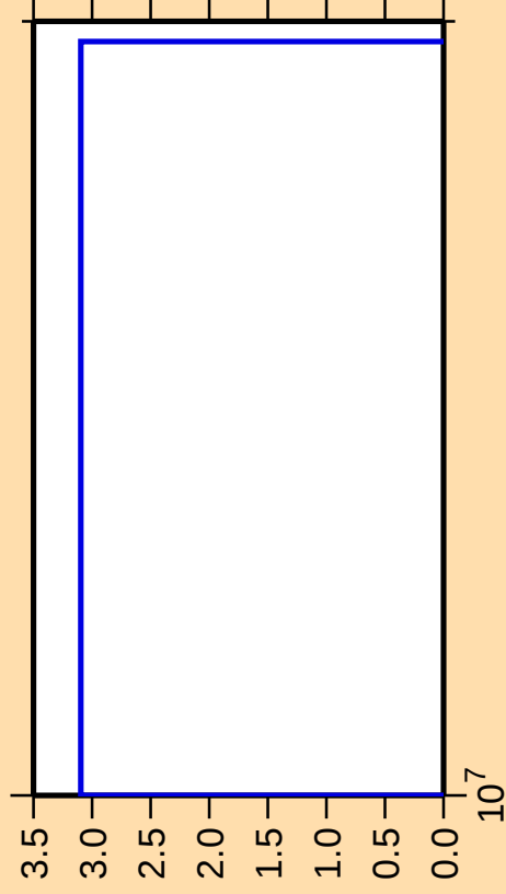
\Delta\sigma/\sigma vs. E for ^{77}\text{Ge}(n,2n\alpha)
