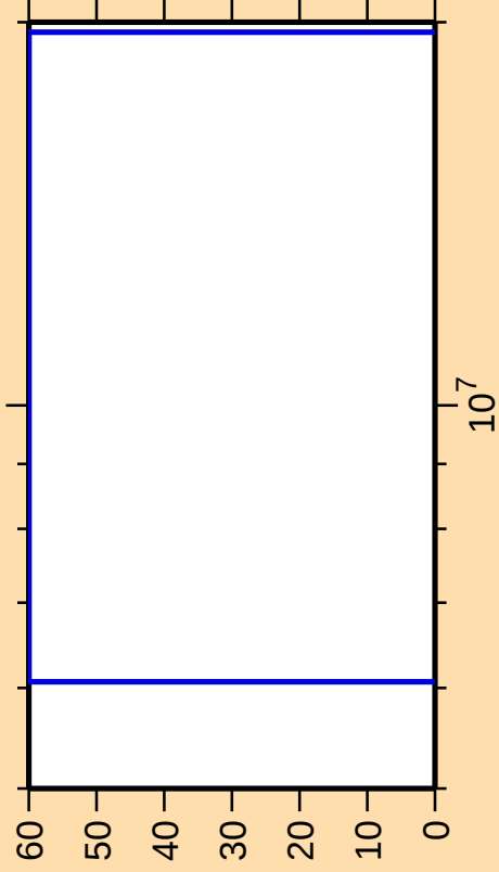
\Delta\sigma/\sigma vs. E for ^{77}\text{Ge}(n,\gamma)
