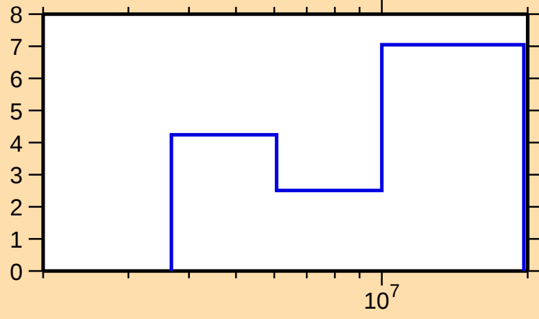
\Delta\sigma/\sigma vs. E for ^{77}\text{Ge}(n,\text{tot.})
