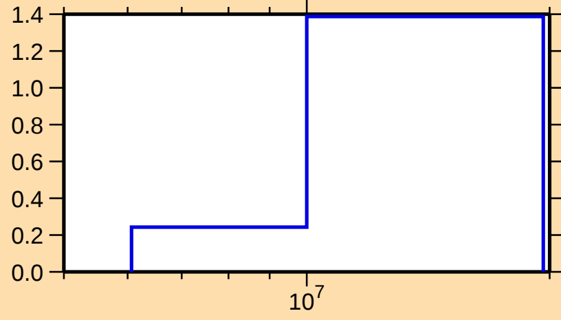
\sigma vs. E for ^{77}\text{Ge}(n,2n)
