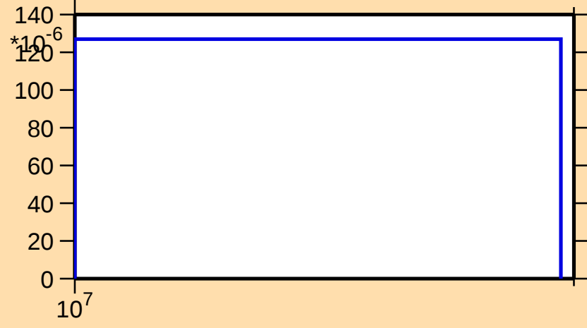
\sigma vs. E for ^{77}\text{Ge}(n,d)
