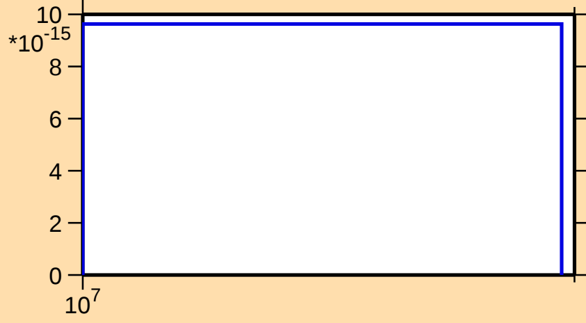
\sigma vs. E for ^{77}\text{Ge}(n,\text{nt})
