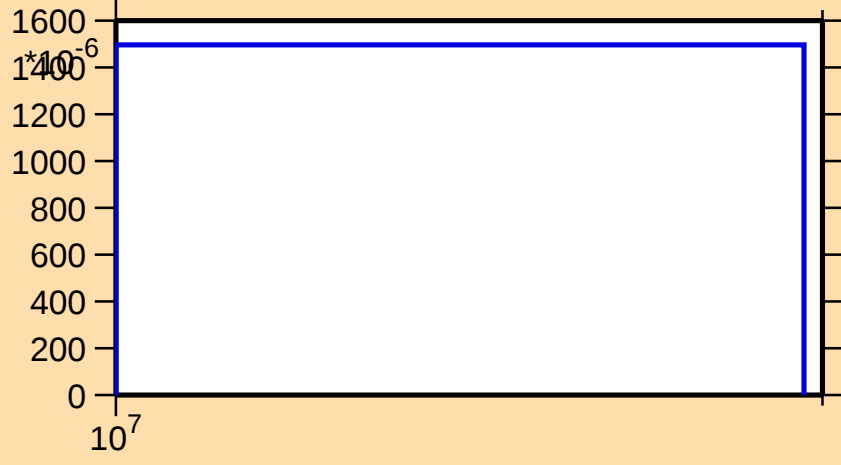
\sigma vs. E for ^{77}\text{Ge}(n,3n)
