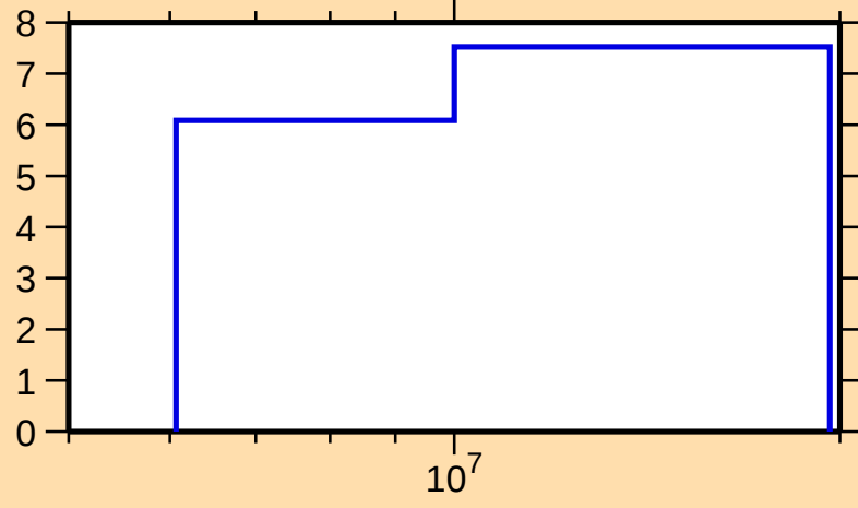
\Delta\sigma/\sigma vs. E for ^{77}\text{Ge}(n,\text{el.})
