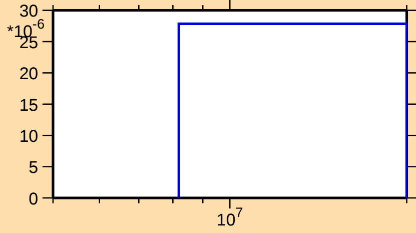
\sigma vs. E for ^{77}\text{Ge}(n,np)
