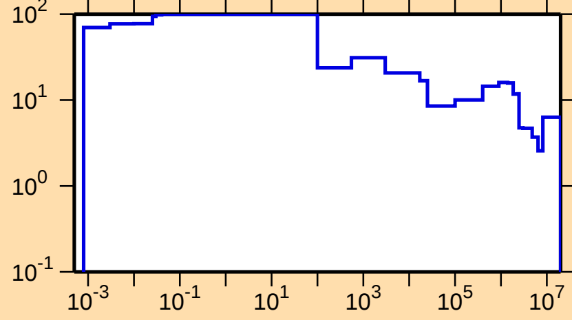
\Delta\sigma/\sigma vs. E for ^{77}\text{Ge}(n,\text{tot.})
