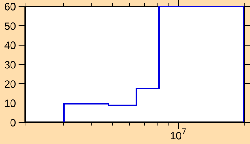
\Delta\sigma/\sigma vs. E for ^{77}\text{Ge}(n,n\text{cont.})
