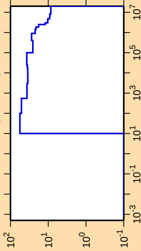
\Delta\sigma/\sigma vs. E for ^{77}\text{Ge}(n,\text{nonel.})
