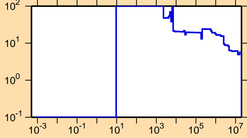
\Delta\sigma/\sigma vs. E for ^{77}\text{Ge}(n,\text{nonel.})
