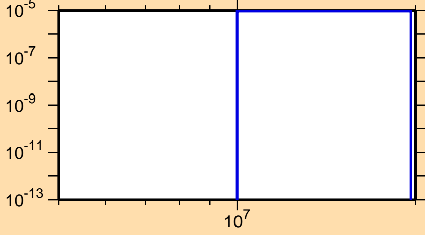
\sigma vs. E for ^{77}\text{Ge}(n,t)
