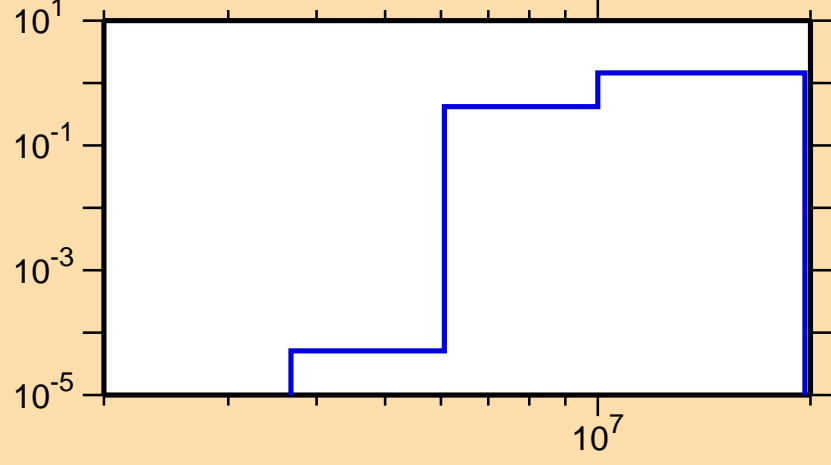
\sigma vs. E for ^{77}\text{Ge}(n,2n)
