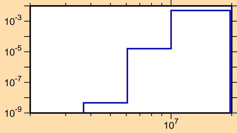
\sigma vs. E for ^{77}\text{Ge}(n,p)
