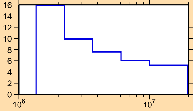
\Delta\sigma/\sigma vs. E for ^{77}\text{Ge}(n,n\text{onel.})
