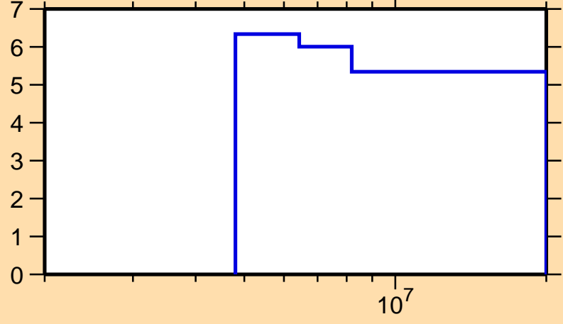
\Delta\sigma/\sigma vs. E for ^{77}\text{Ge}(n,\text{nonel.})
