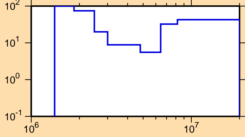
\Delta\sigma/\sigma vs. E for ^{77}\text{Ge}(n,n\text{cont.})
