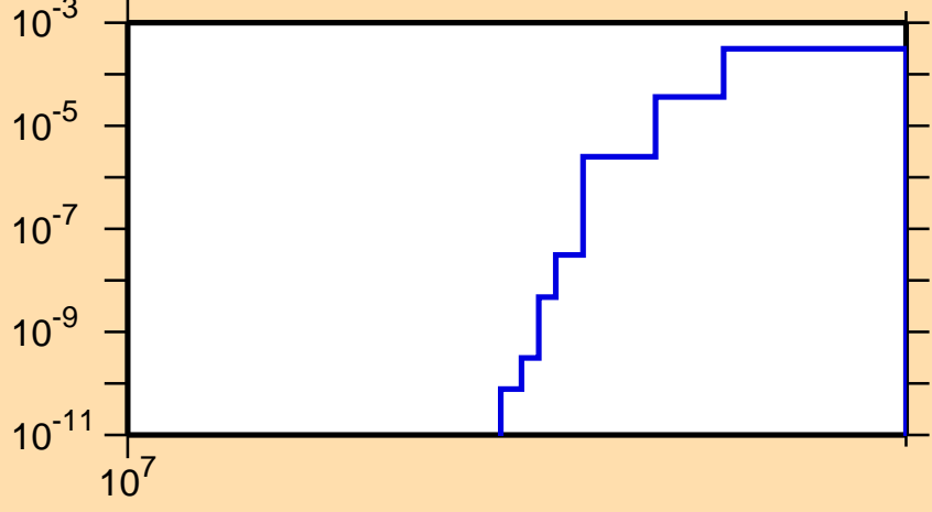
\sigma vs. E for ^{78}\text{Ge}(n,np)
