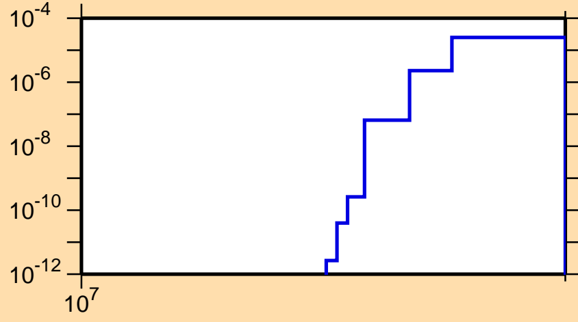
\sigma vs. E for ^{78}\text{Ge}(n,t)
