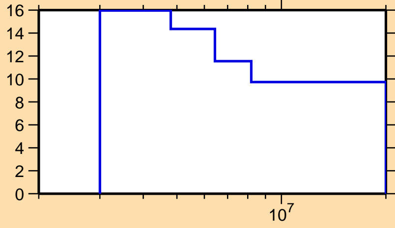
\Delta\sigma/\sigma vs. E for ^{78}\text{Ge}(n,n\text{onl.})
