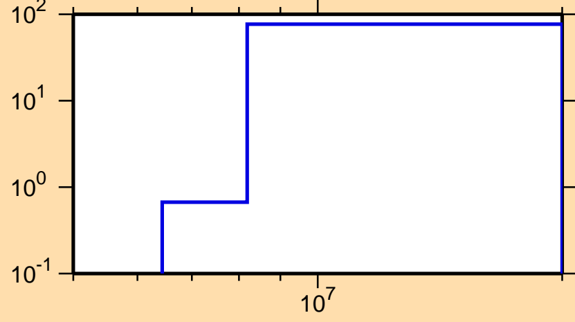
\Delta\sigma/\sigma vs. E for ^{78}\text{Ge}(n,p)
