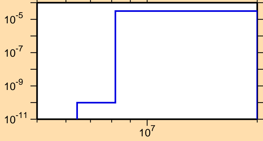
\sigma vs. E for ^{78}\text{Ge}(n,\alpha)
