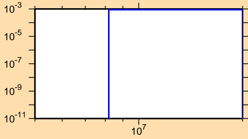
\sigma vs. E for ^{78}\text{Ge}(n,p)
