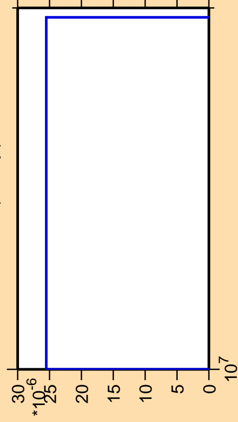
\Delta\sigma/\sigma vs. E for ^{79}\text{Ge}(n,2np)
