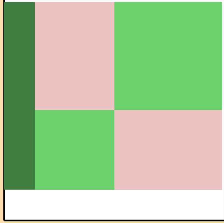
\Delta\sigma/\sigma vs. E for ^{79}\text{Ge}(n,n_1)
