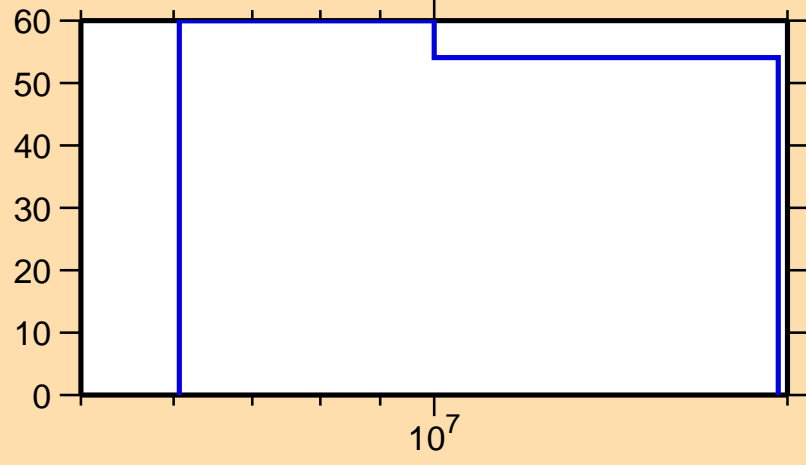
\Delta\sigma/\sigma vs. E for ^{79}\text{Ge}(n,n\text{cont.})
