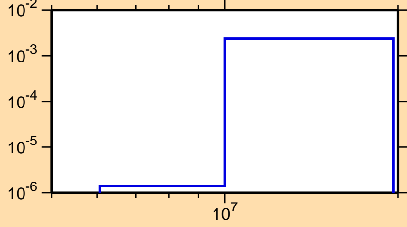
\sigma vs. E for ^{79}\text{Ge}(n,p)
