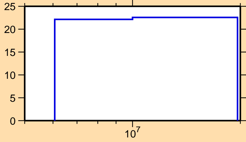
\Delta\sigma/\sigma vs. E for ^{79}\text{Ge}(n,el.)
