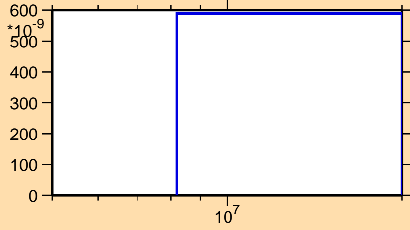
\sigma vs. E for ^{79}\text{Ge}(n,\alpha)
