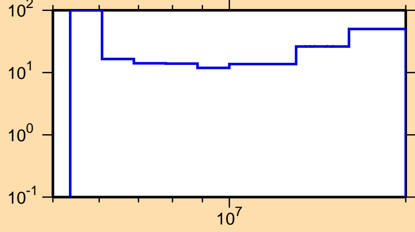
\Delta\sigma/\sigma vs. E for ^{79}\text{Ge}(n,2n)
