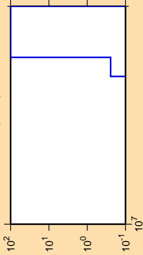
\Delta\sigma/\sigma vs. E for ^{79}\text{Ge}(n,nd)
