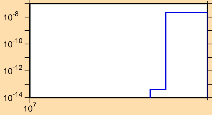
\sigma vs. E for ^{79}\text{Ge}(n,nd)
