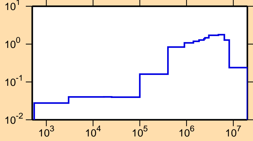
\sigma vs. E for ^{79}\text{Ge}(n,\text{inel.})
