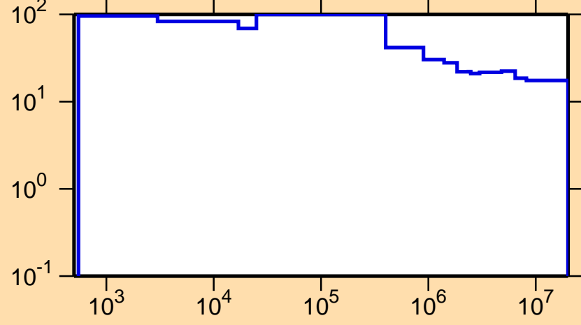
\Delta\sigma/\sigma vs. E for ^{79}\text{Ge}(n,\text{nonel.})
