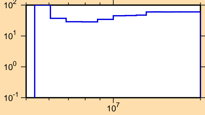
\Delta\sigma/\sigma vs. E for ^{80}\text{Ge}(n,n\text{cont.})
