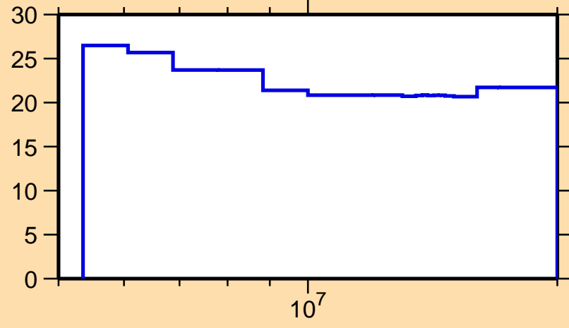
\Delta\sigma/\sigma vs. E for ^{80}\text{Ge}(n,n\text{onel.})
