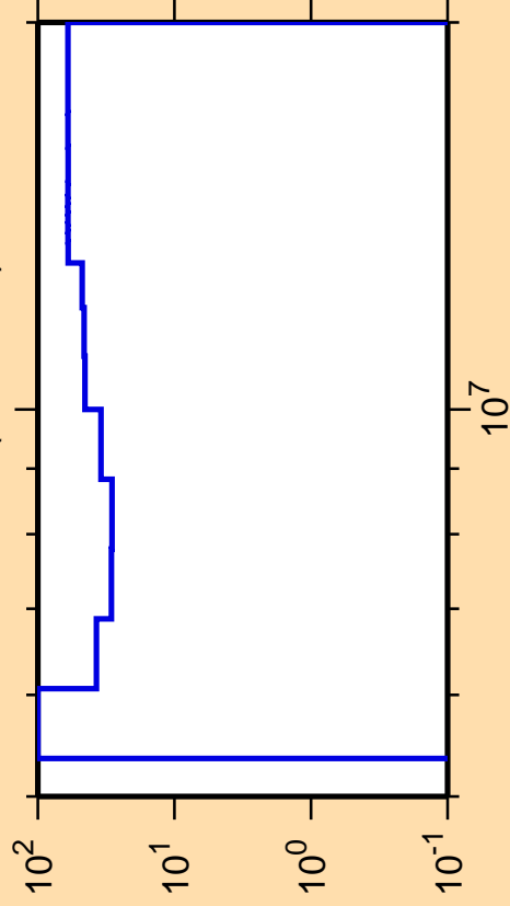
\Delta\sigma/\sigma vs. E for ^{80}\text{Ge}(n,\text{ncont.})
