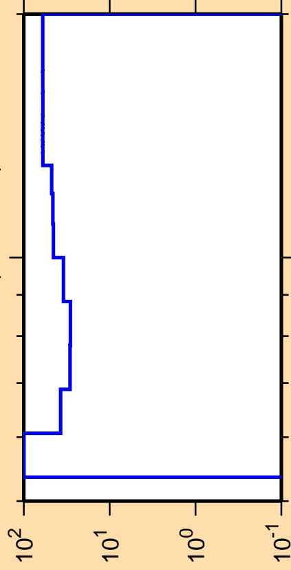
\Delta\sigma/\sigma vs. E for ^{80}\text{Ge}(n,\text{ncont.})
