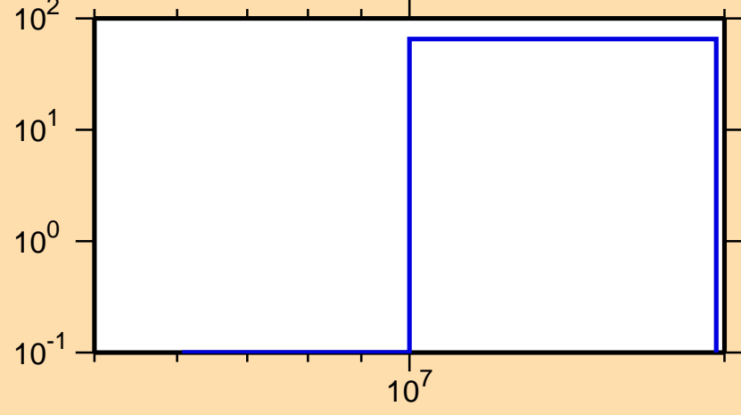
\Delta\sigma/\sigma vs. E for ^{80}\text{Ge}(n,p)
