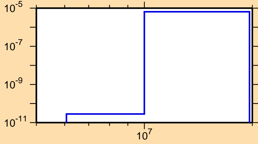
\sigma vs. E for ^{80}\text{Ge}(n,\alpha)
