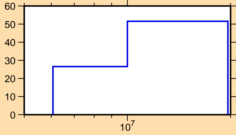
\Delta\sigma/\sigma vs. E for ^{80}\text{Ge}(n,ncont.)
