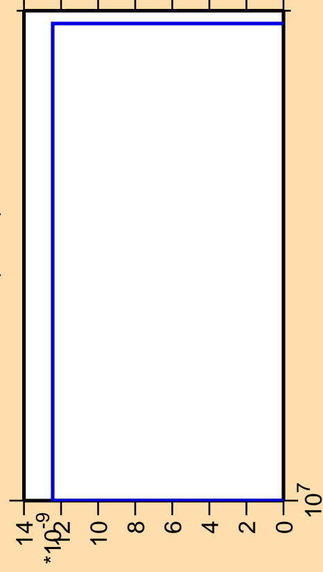
\Delta\sigma/\sigma vs. E for ^{80}\text{Ge}(n,\text{nd})
