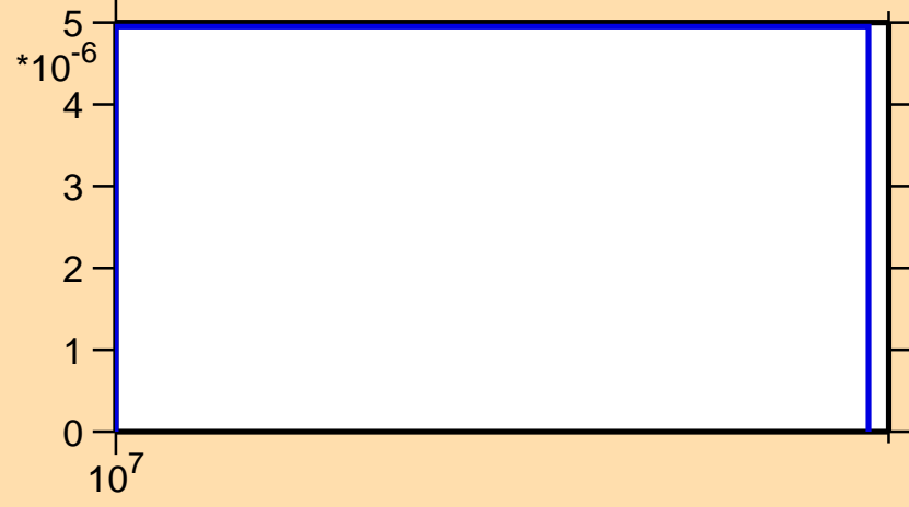
\sigma vs. E for ^{80}\text{Ge}(n,d)
