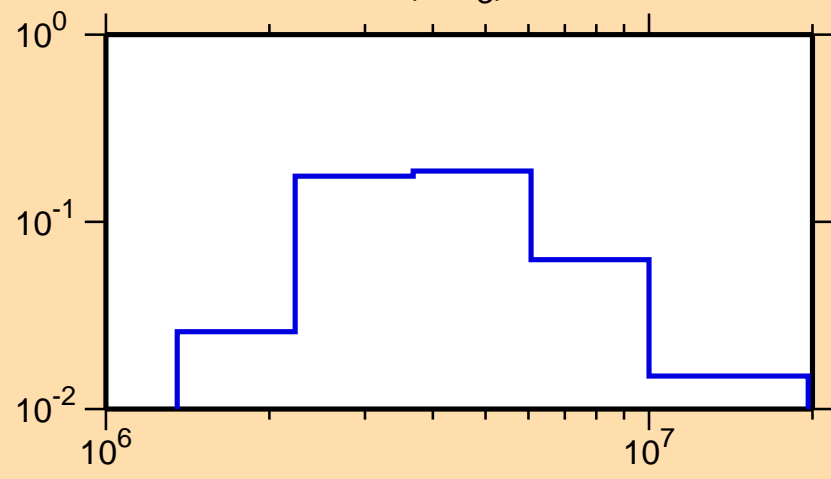
\sigma vs. E for ^{80}\text{Ge}(n,n_3)
