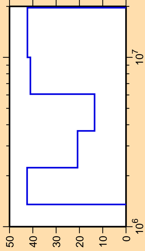
\Delta\sigma/\sigma vs. E for ^{80}\text{Ge}(n,n_3)
