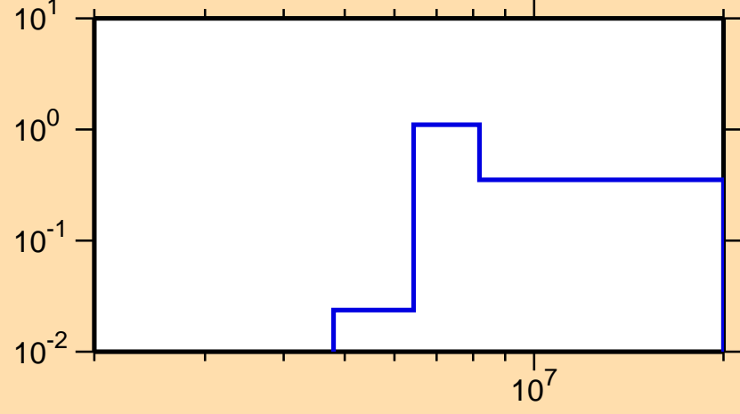
\sigma vs. E for ^{80}\text{Ge}(n,n\text{cont.})
