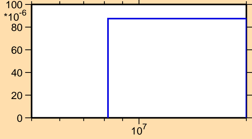
\sigma vs. E for ^{80}\text{Ge}(n,p)
