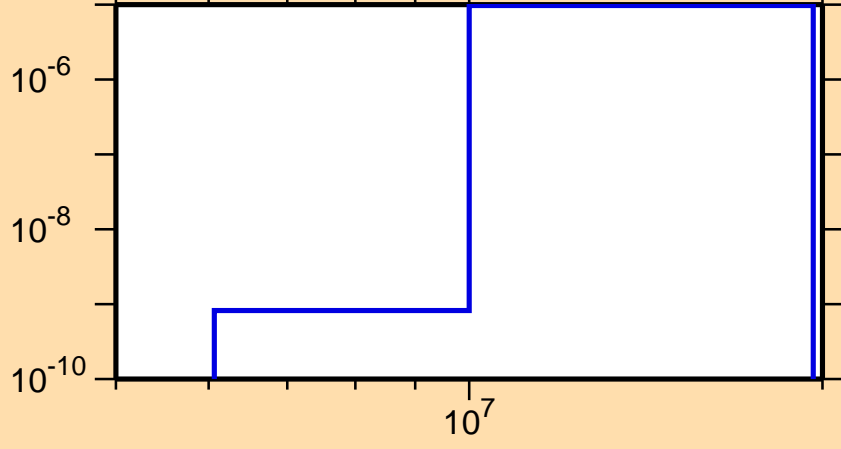
\sigma vs. E for ^{81}\text{Ge}(n,\alpha)
