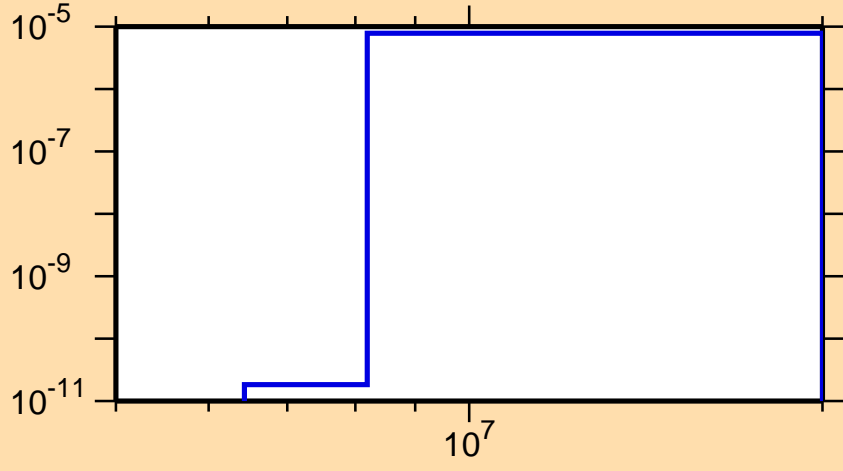
\sigma vs. E for ^{81}\text{Ge}(n,\alpha)
