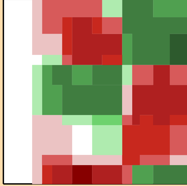
\Delta\sigma/\sigma vs. E for ^{81}\text{Ge}(n,n\text{cont.})
