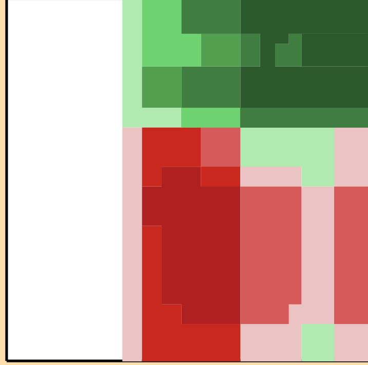
\Delta\sigma/\sigma vs. E for ^{82}\text{Ge}(n,n\text{cont.})
