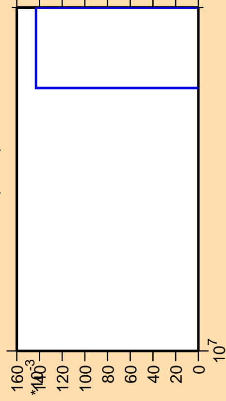
\Delta\sigma/\sigma vs. E for ^{82}\text{Ge}(n,\text{nd})
