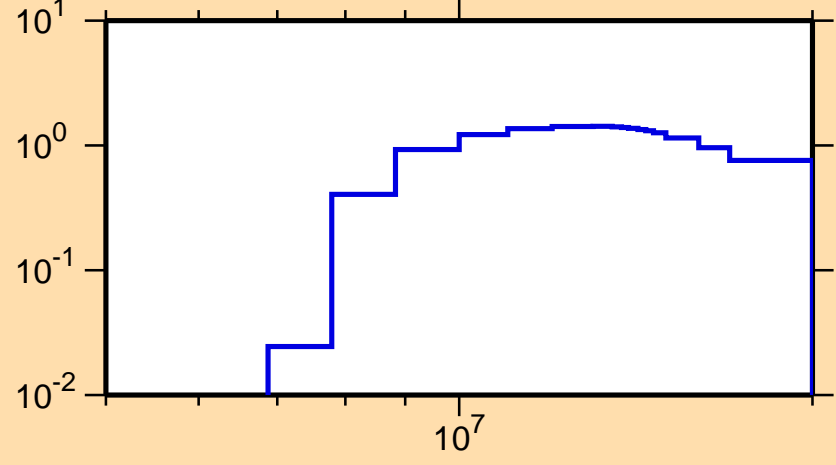
\sigma vs. E for ^{82}\text{Ge}(n,2n)
