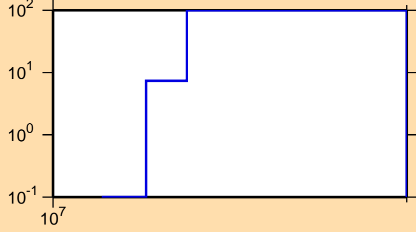
\Delta\sigma/\sigma vs. E for ^{82}\text{Ge}(n,p)
