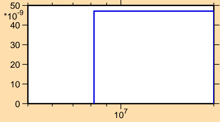
\sigma vs. E for ^{82}\text{Ge}(n,np)
