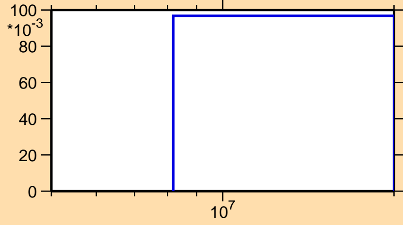
\sigma vs. E for ^{82}\text{Ge}(n,3n)
