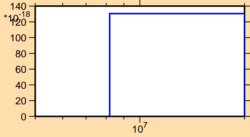
\sigma vs. E for ^{82}\text{Ge}(n,nd)
