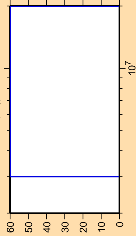
\Delta\sigma/\sigma vs. E for ^{82}\text{Ge}(n,\gamma)
