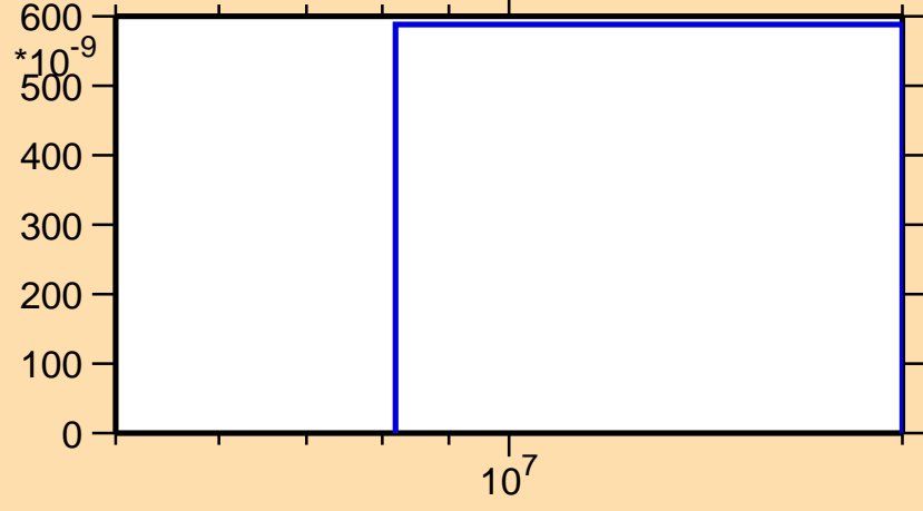
\sigma vs. E for ^{82}\text{Ge}(n,\alpha)
