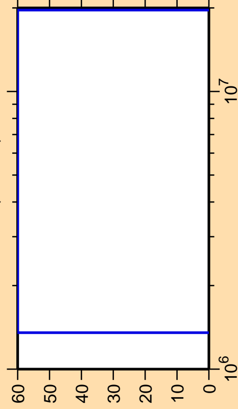
\Delta\sigma/\sigma vs. E for ^{154}\text{Hf}(n,\text{inel.})
