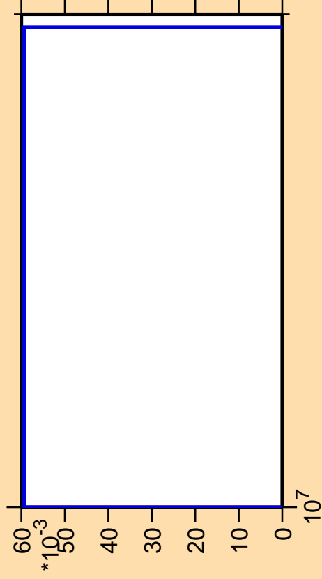
\Delta\sigma/\sigma vs. E for ^{154}\text{Hf}(n,2n\alpha)
