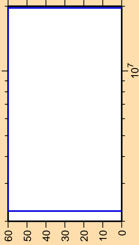
\Delta\sigma/\sigma vs. E for ^{154}\text{Hf}(n,\text{ncont.})
