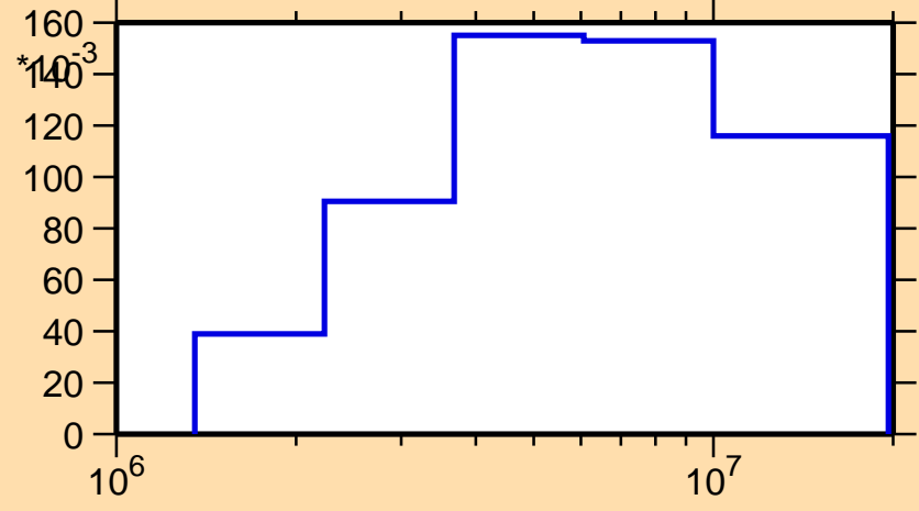
\sigma vs. E for ^{154}\text{Hf}(n,\text{inel.})
