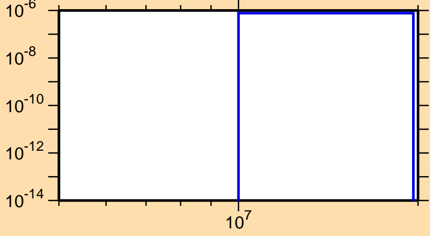
\sigma vs. E for ^{154}\text{Hf}(n,\text{pt})
