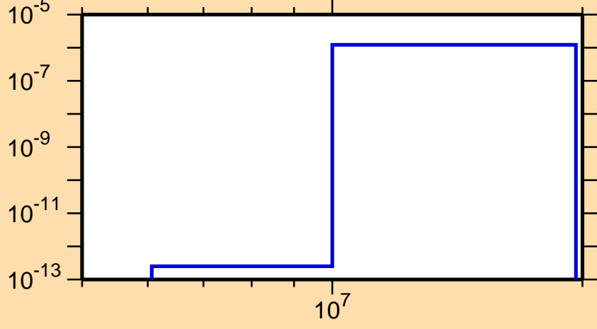
\sigma vs. E for ^{154}\text{Hf}(\text{mt } 45)
