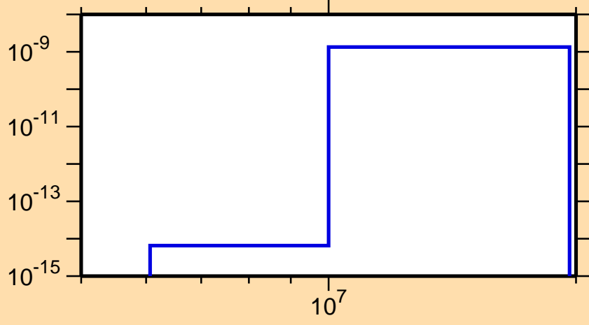
\sigma vs. E for ^{154}\text{Hf}(\text{mt117})
