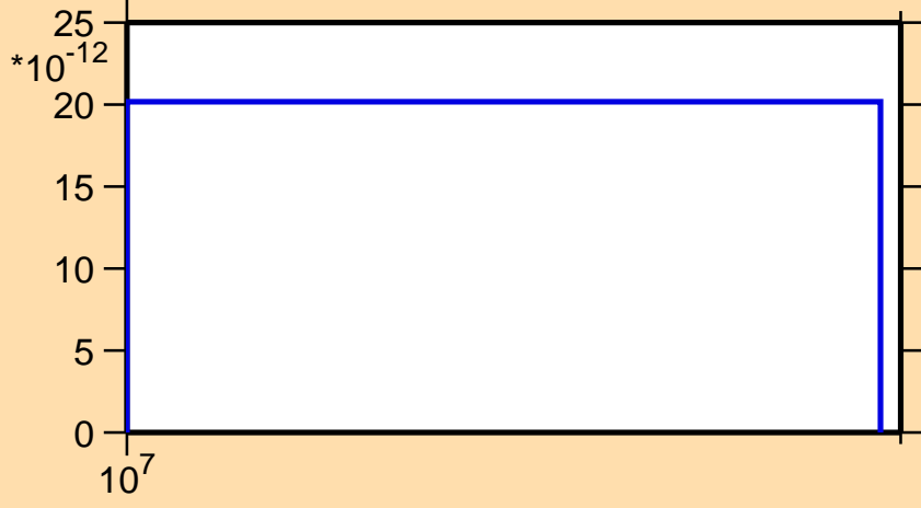
\sigma vs. E for ^{154}\text{Hf} (mt 34)
