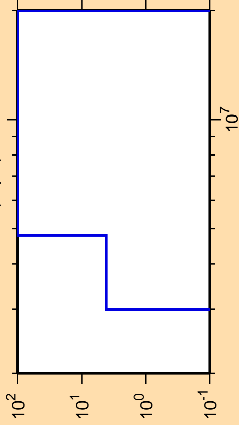
\Delta\sigma/\sigma vs. E for ^{154}\text{Hf}(n,\text{pd})
