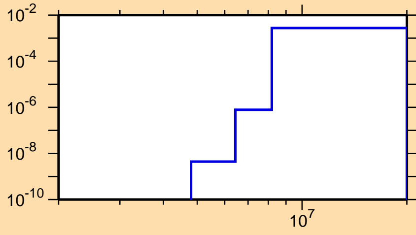
\sigma vs. E for ^{154}\text{Hf}(n,\text{pd})
