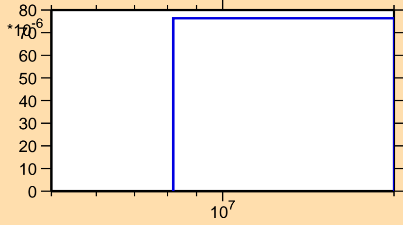
\sigma vs. E for ^{154}\text{Hf}(n,2n)
