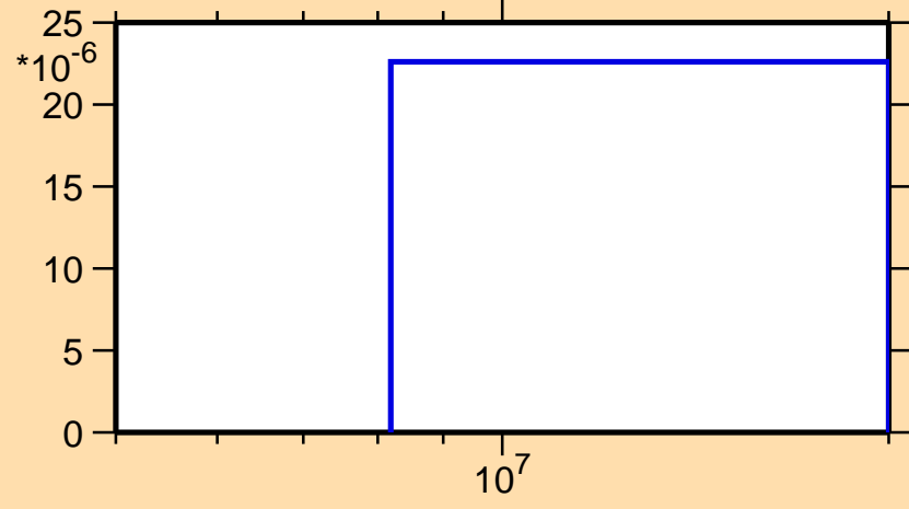
\sigma vs. E for ^{154}\text{Hf}(n,t)
