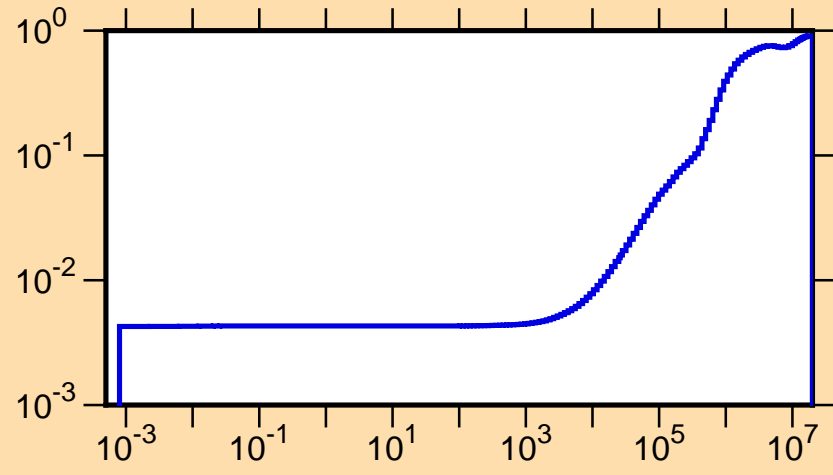
\mu vs. E for ^{158}\text{Hf}(\text{mt251})
