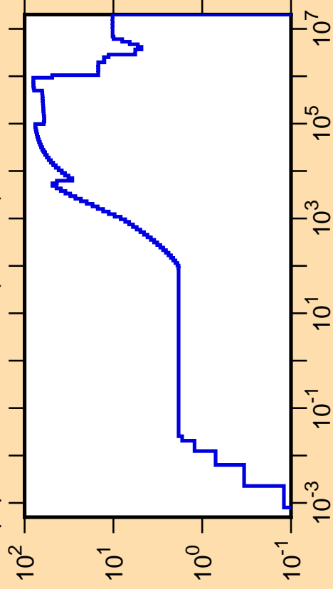
\Delta\mu/\mu vs. E for ^{158}\text{Hf}(\text{mt251})
