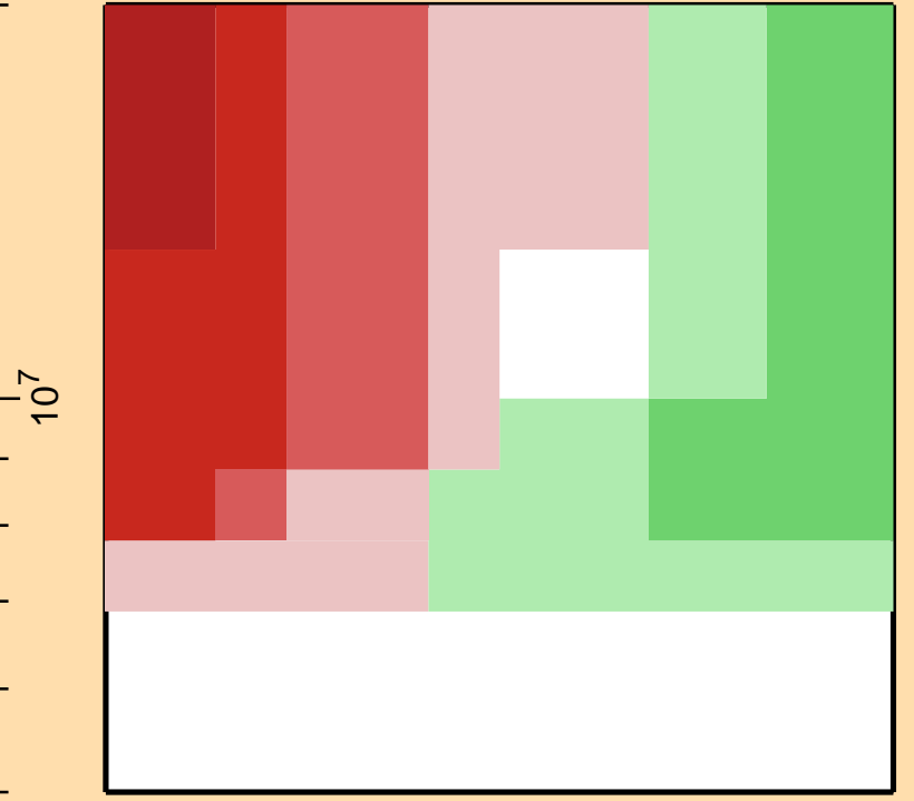
Correlation Matrix
