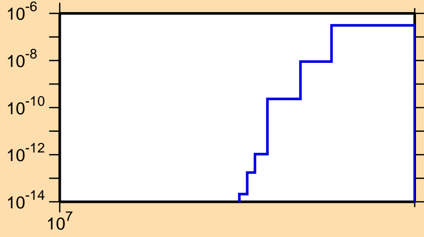
\sigma vs. E for ^{158}\text{Hf}(n,nd)
