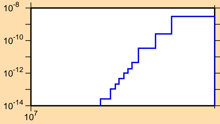
\sigma vs. E for ^{158}\text{Hf}(\text{mt } 34)
