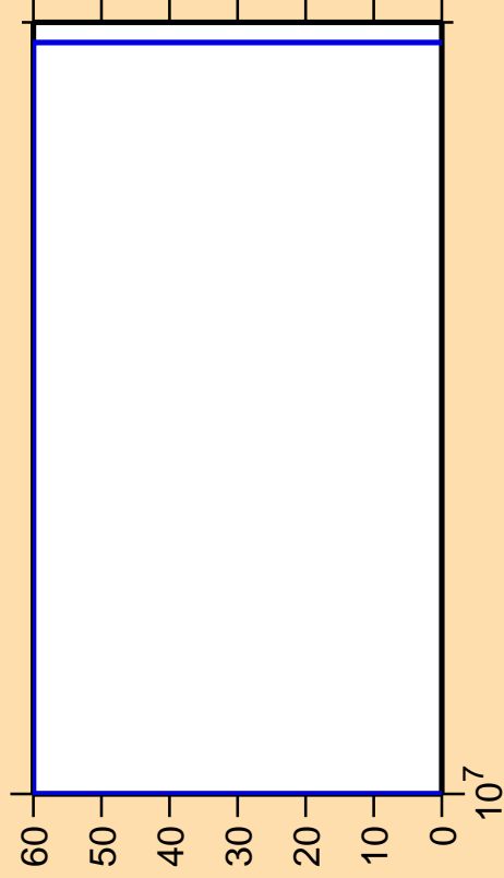
\Delta\sigma/\sigma vs. E for ^{158}\text{Hf} (mt 34)
