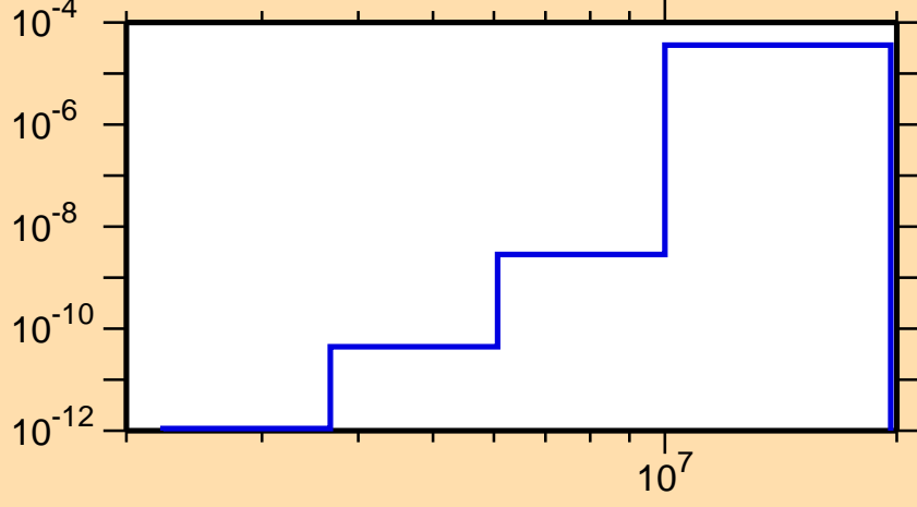
\sigma vs. E for ^{158}\text{Hf}(n,\text{He3})
