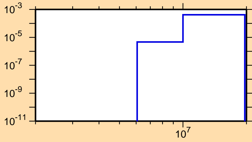
\sigma vs. E for ^{158}\text{Hf} (mt 45)
