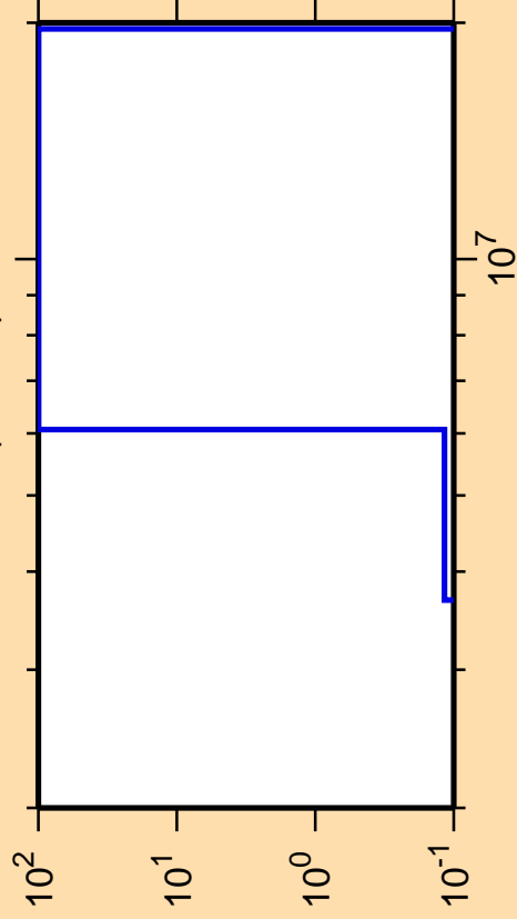
\Delta\sigma/\sigma vs. E for ^{158}\text{Hf} (mt 45)
