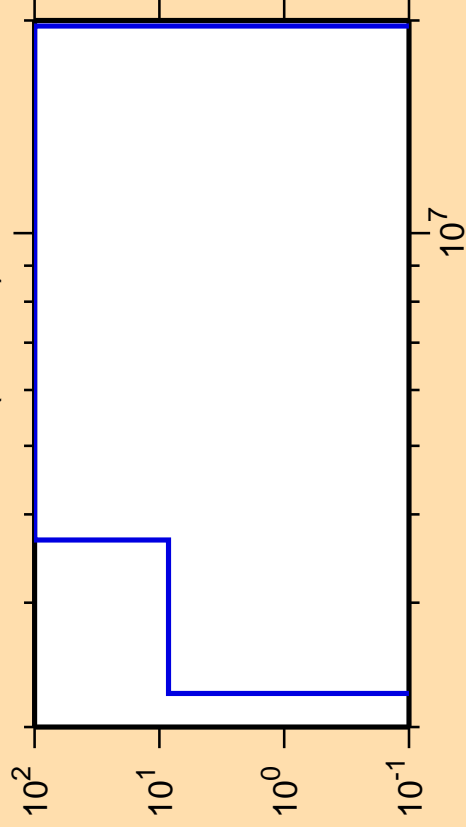
\Delta\sigma/\sigma vs. E for ^{158}\text{Hf}(n,\text{He3})
