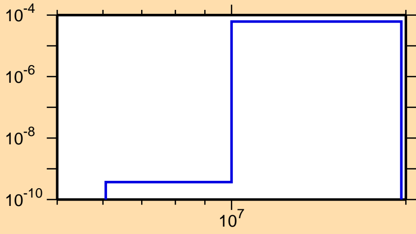
\sigma vs. E for ^{158}\text{Hf}(n,\text{pd})
