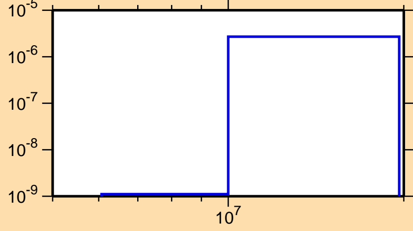
\sigma vs. E for ^{158}\text{Hf}(\text{mt117})
