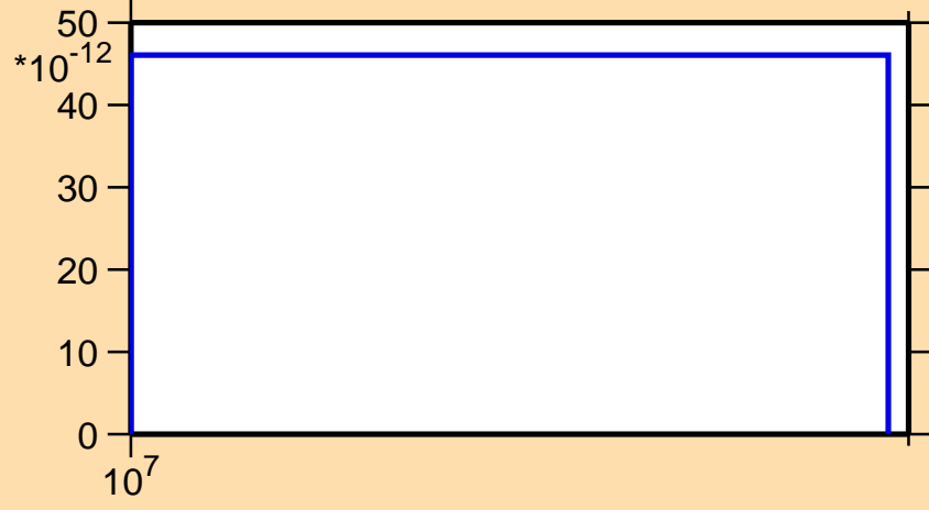
\sigma vs. E for ^{158}\text{Hf} (mt 34)
