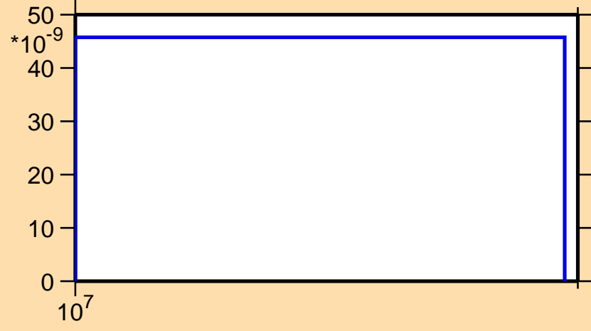
\sigma vs. E for ^{158}\text{Hf}(n,\text{pt})
