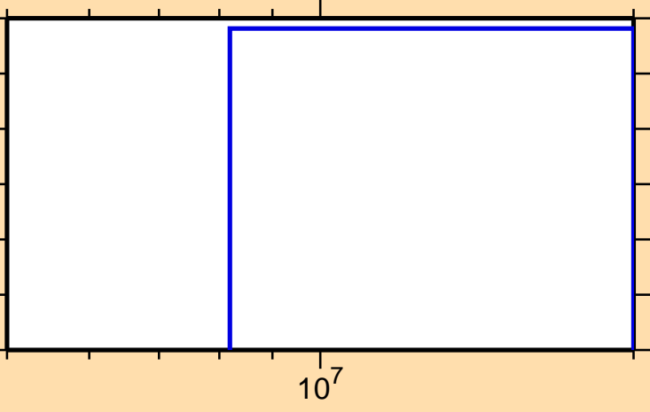
\sigma vs. E for ^{158}\text{Hf}(n,\text{nd})
