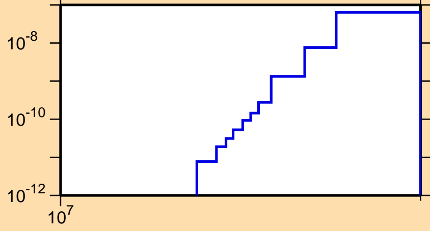
\sigma vs. E for ^{159}\text{Hf}(\text{mt } 34)
