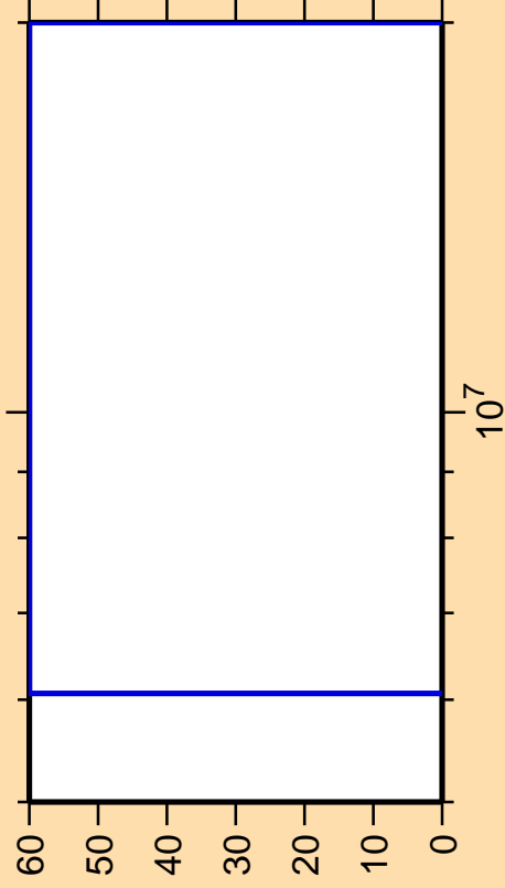
\Delta\sigma/\sigma vs. E for ^{159}\text{Hf}(n, ncont.)
