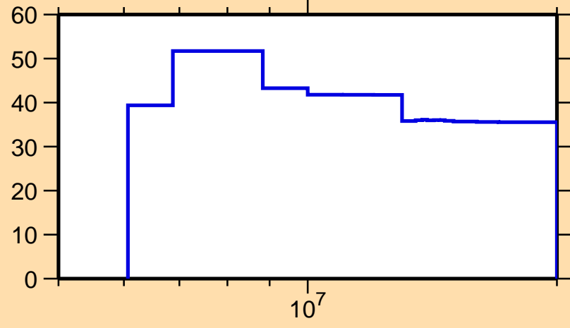
\Delta\sigma/\sigma vs. E for ^{159}\text{Hf}(n, el.)
