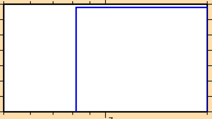
\sigma vs. E for ^{159}\text{Hf}(n,2np)
