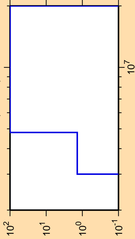
\Delta\sigma/\sigma vs. E for ^{159}\text{Hf}(n,\text{He3})
