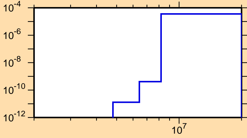
\sigma vs. E for ^{159}\text{Hf}(n,\text{He3})
