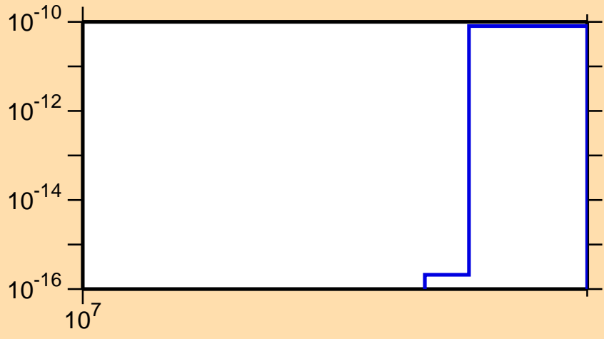
\sigma vs. E for ^{161}\text{Hf}(n,nt)
