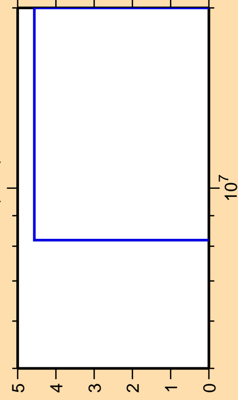
\Delta\sigma/\sigma vs. E for ^{161}\text{Hf}(n,nt)
