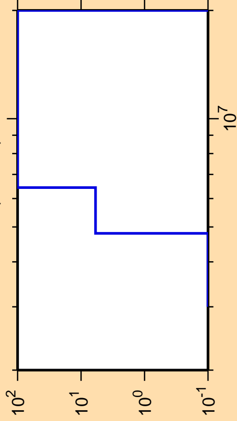
\Delta\sigma/\sigma vs. E for ^{161}\text{Hf}(n,\text{He}3)
