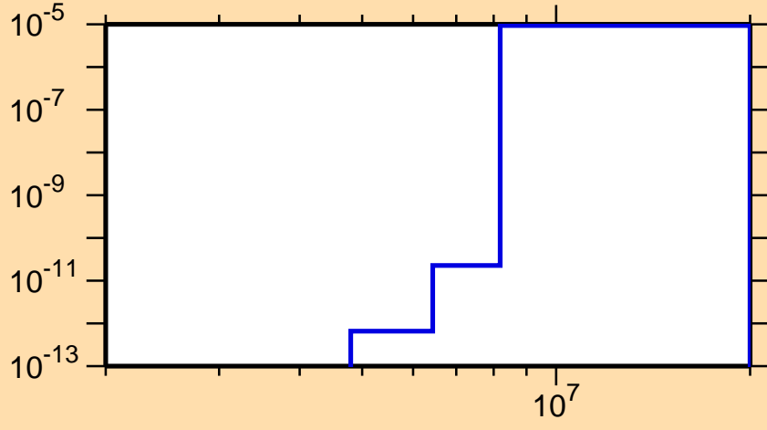
\sigma vs. E for ^{161}\text{Hf}(n,\text{He}3)
